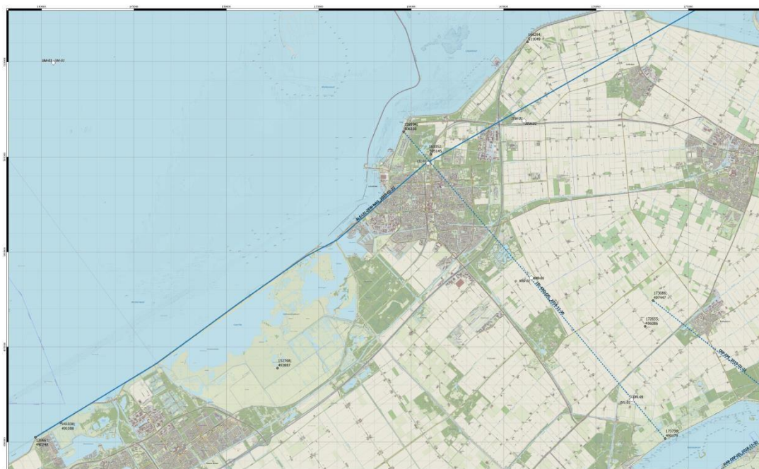
Planned Seismic Lines Area A, B, H, I Part 3 of 8 - 1:50.000 0 2 4 6 8 10 km CRS: RD New (Amersfoort; 28992)
