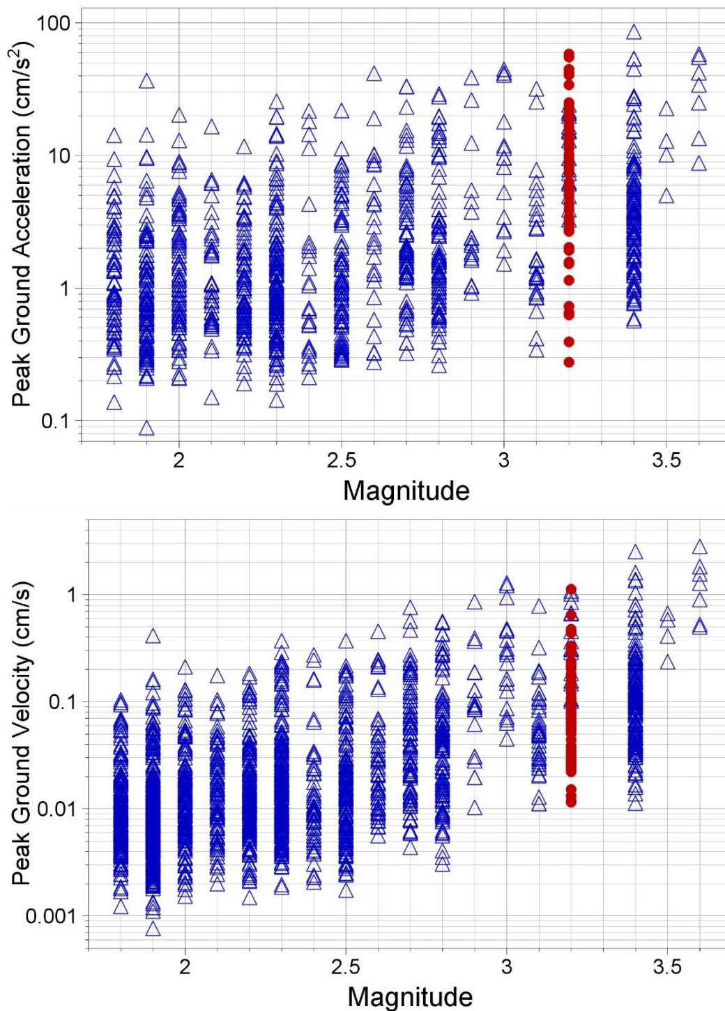
Figure 2.8 Geometric mean horizontal components of PGA (upper) and PGV (lower) recorded during the Garrelswear earthquake (red) and in previous earthquakes (blue) plotted against local magnitude.
