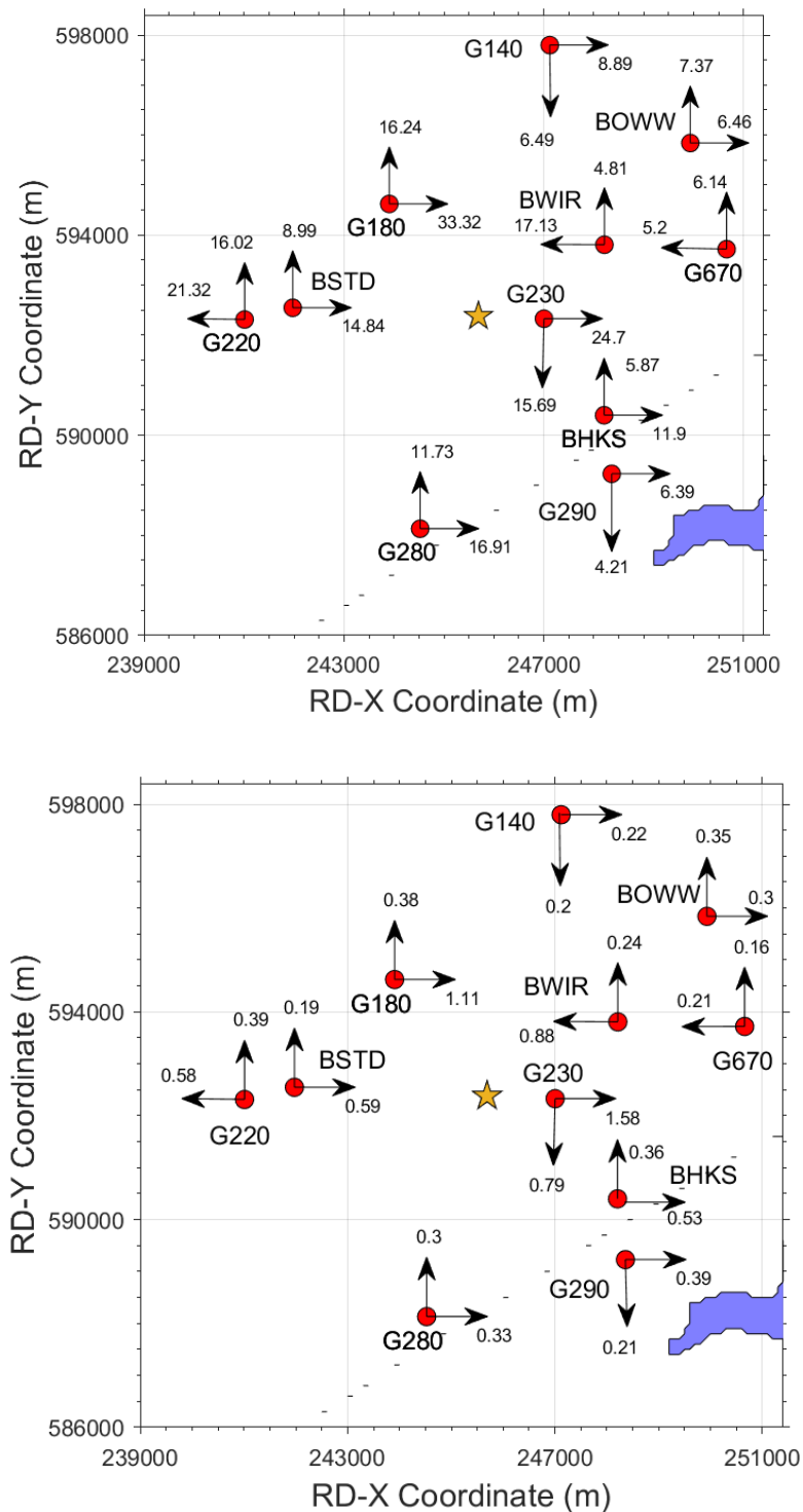
Figure 2.7 Horizontal components of PGA (upper) and PGV (lower) recorded during the Garrelsweer earthquake at epicentral distances of less than 6 km; units are cm/s 2 and cm/s, respectively.
