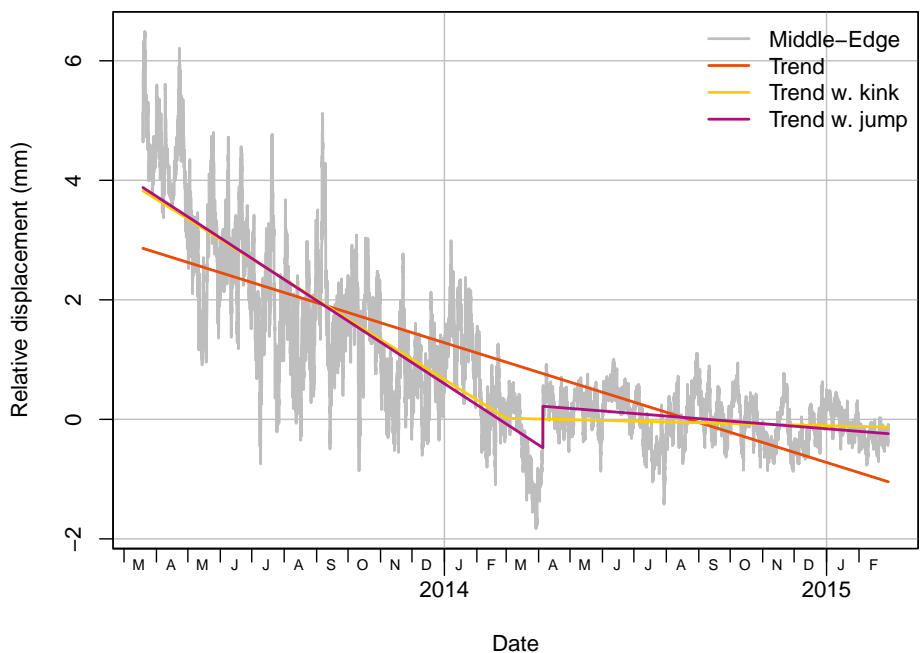
Figure 12 The fitted models, with either a jump or a kink, to the data as processed by the TU Delft without any additional filtering by Statistics Netherlands for the best-fitting position of that break in the linear model fit of the difference between the group averages of 'Middle' and 'Edge'.
