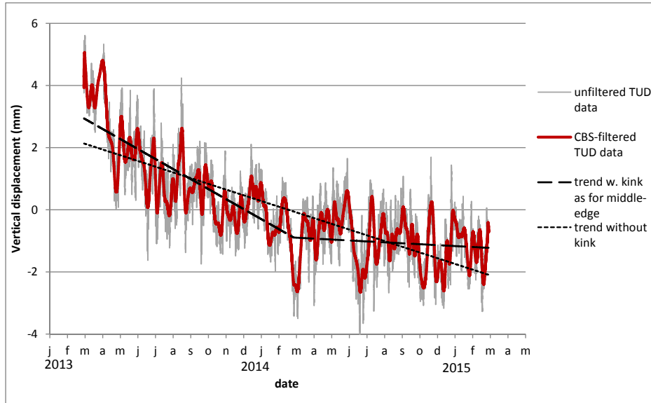
Figure 13 The fitted models, with or without a kink, to the Ten Post - Veendam time series as processed by the TU Delft without any additional filtering. Grey : the TUD data, red line: the time series that results if the filter used by Statistics Netherlands is applied. Black dashed lines, fits to the TUD data without applying the filtering procedure of Statistics Netherlands.
