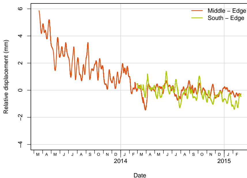
Figure 9 The time series of the TU Delft processed GPS height data, and after filtering, for the differences between the group averages 'Middle' – 'Edge' (in red), and 'South' – 'Edge' (in green). Note that the vertical scale is in mm.
