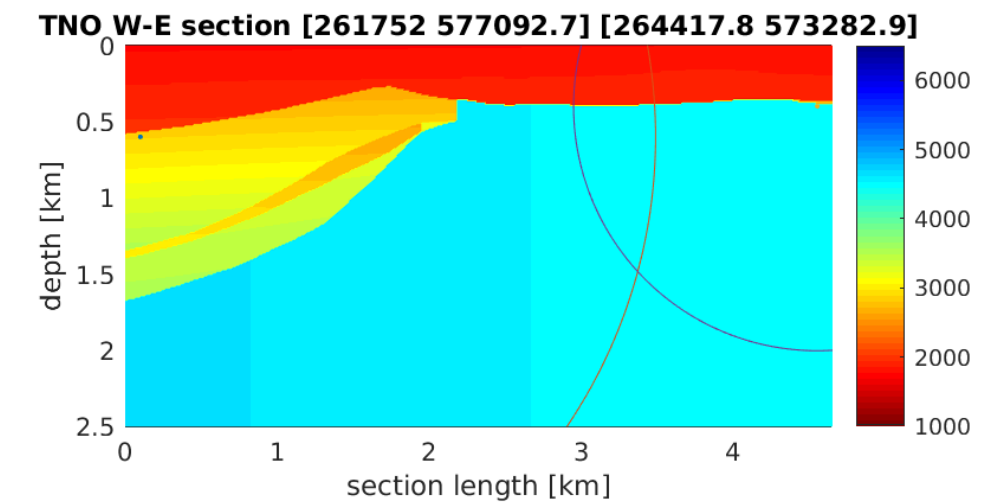
Fig. 10: Section through Velmod-3 (Dalfsen et al., 2006) between stations G52 and G57 of the KNMI network. The colour map shows P-wave velocities. Blue correspond to mostly halite deposited in Perm, yellow to green corresponds to chalk from the Cretaceous and red corresponds to mostly unconsolidated sediments from the Paleogene and Neogene. The red and blue line show P-S delay isochrones for geophones G524 and G574, respectively. The intersection of the two lines is an estimate of the hypocentre.
