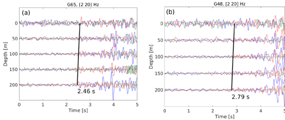
Fig. 6 (a) 3-component response at 5 depth levels in boreholes (a) G65 and (b) G48. The red, blue and green seismograms denote the vertical, radial and transverse particle velocity recordings. Thick black lines denote depth-consistent picks of the first P-wave onset. Geophone G653 (depth level 150 m) has malfunctioning horizontal components.
