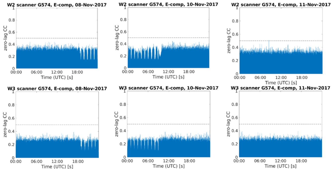
Fig. B.2: Template matching from day of year (day) 312, 314 and 315. At station G57 there is no data for day 313, and the last part of 312 and the first part of 314 is missing.
