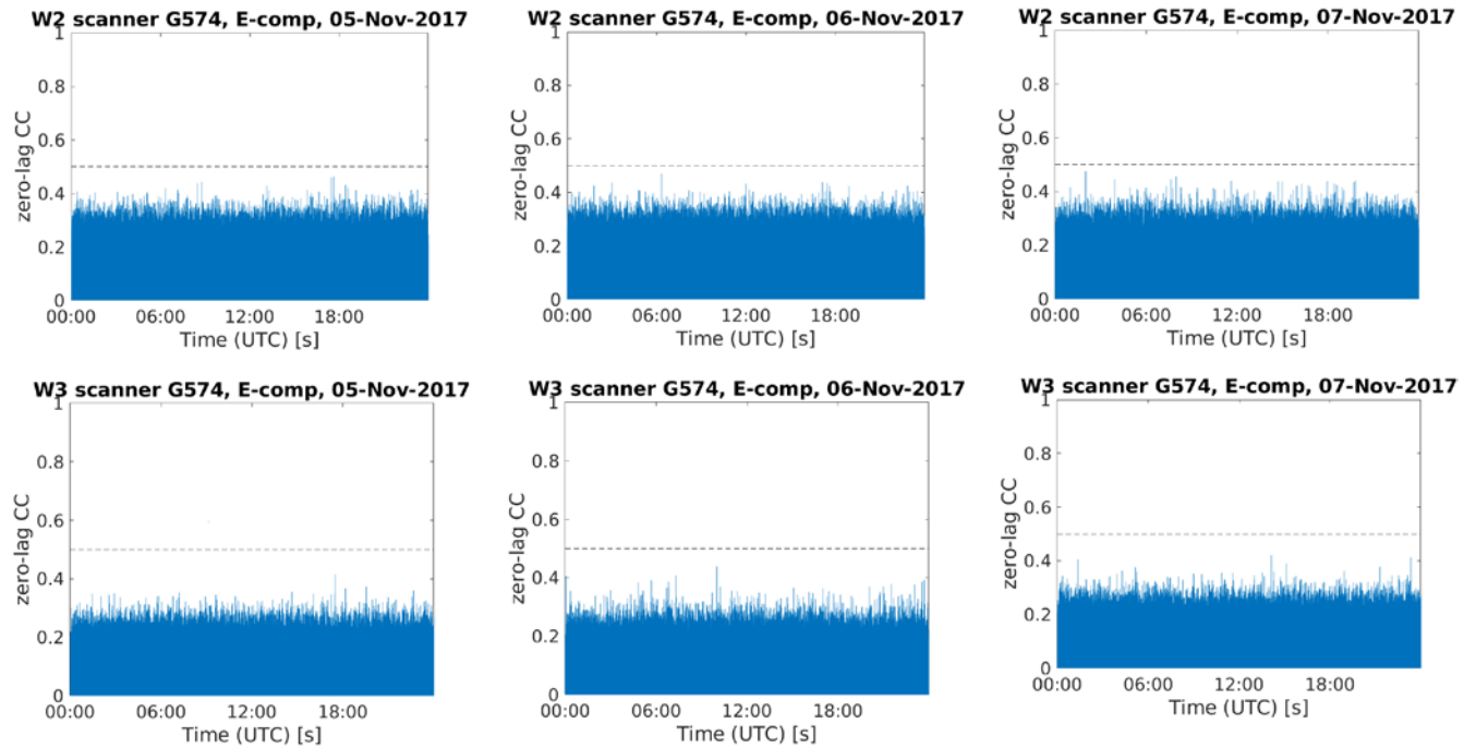
Fig. B.1: Template matching from day of year 309 to 311, with template W2 (upper panels) and W3 (lower panels). The template events have been defined in Fig. 13(a).
