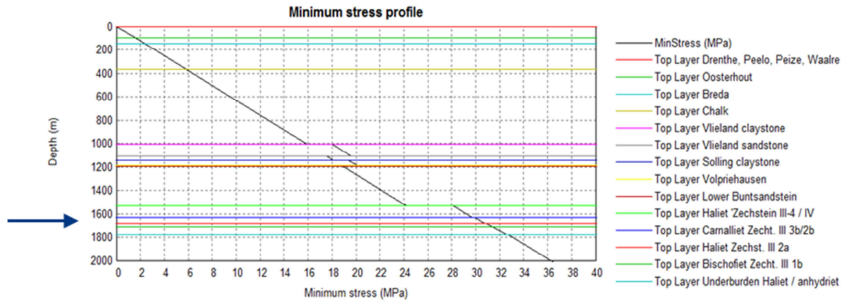
Figure 1. Simplified 'layer-cake' geology of the salt layers plus overburden layers
