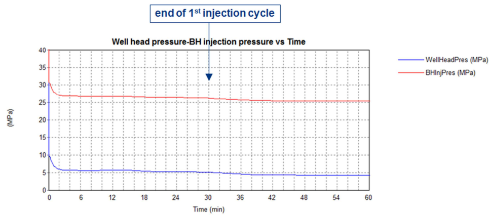
Figure 5a. Computed injection pressures after one hour of injection by simulations using WI/CRI model
