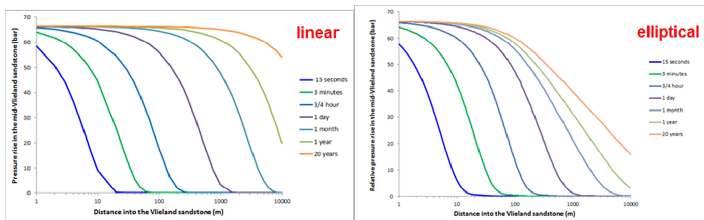
Figure 7. Pore pressure penetration in the Vlieland sandstone
