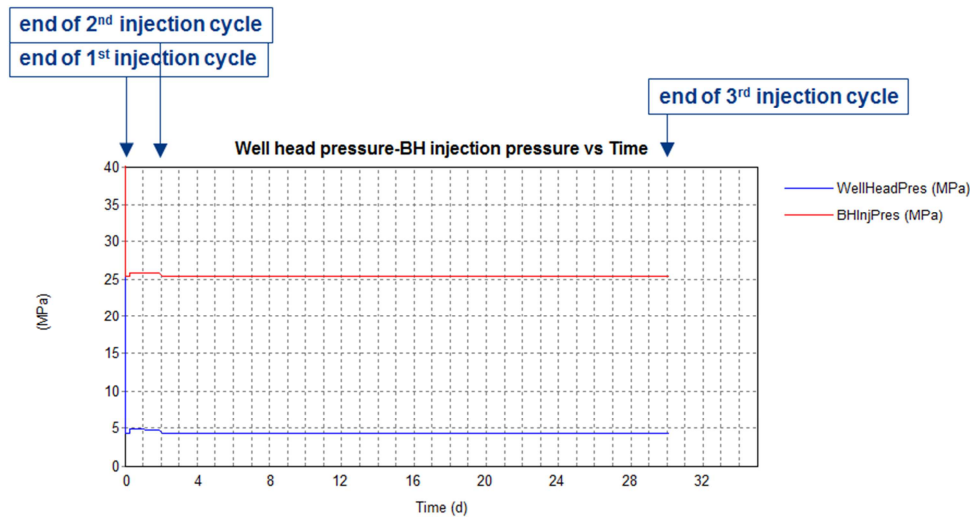
Figure 5c. Computed injection pressures after one month of injection by simulations using WI/CRI model
