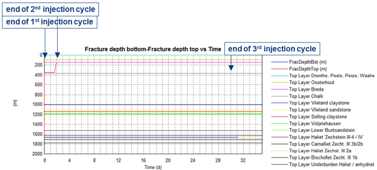
Figure 17b. Results after one month of injection of simulations using WI/CRI model. Low permeability of Vlieland sandstone (30 mD).
