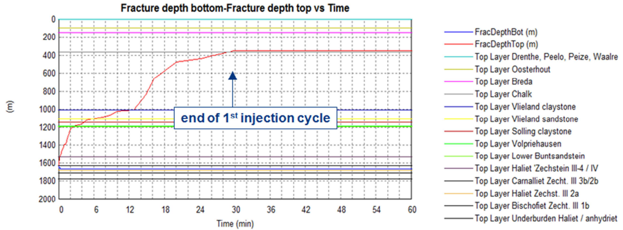
Figure 4a. Results after one hour of injection of simulations using WI/CRI model
