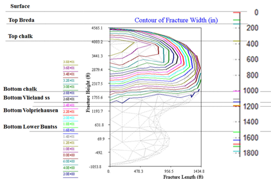
Figure 11. Fracture geometry (plus mesh) after 30 minutes of injection, simulations using BEM model, no stress contrasts between sands and clays
