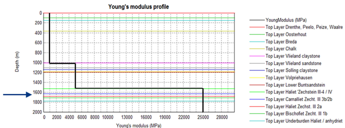
Figure 2. Young's modulus profile
