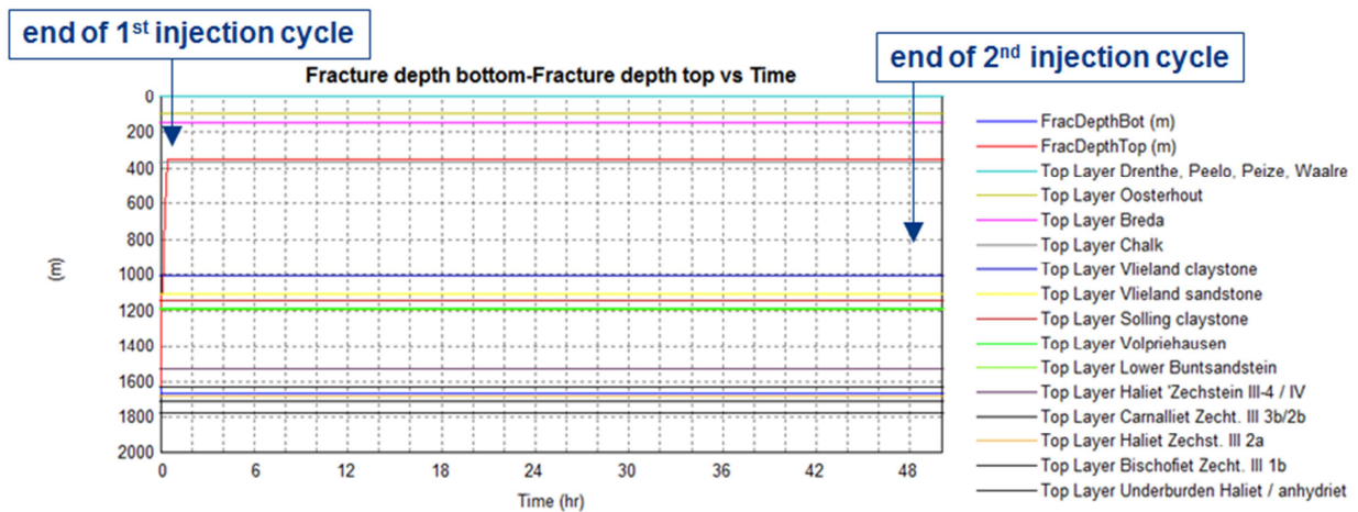
Figure 4b. Results after two days of injection of simulations using WI/CRI model
