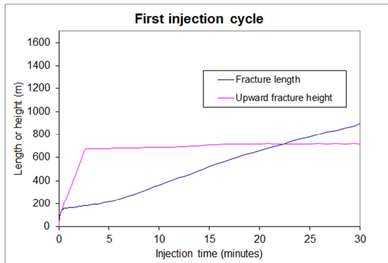
Figure 6b. Fracture growth during first 30 minutes of injection, simulations using BEM model
