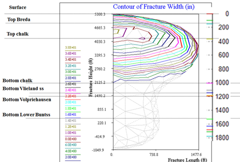
Figure 10a. Fracture geometry (plus mesh) after 28 minutes of injection, simulations using BEM model, no stress contrasts between sands and clays.
