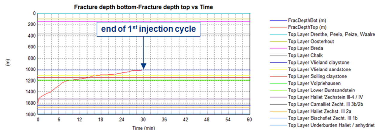
Figure 14. Results after 60 minutes of injection of simulations using WI/CRI model. Low injection rates.
