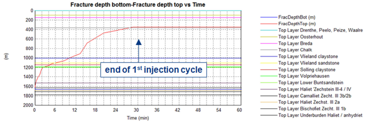
Figure 17a. Results after 60 minutes of injection of simulations using WI/CRI model. Low permeability of Vlieland sandstone (30 mD).
