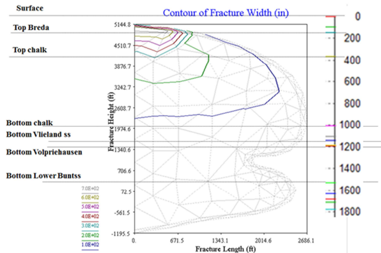
Figure 15. Fracture geometry (plus mesh) after 30 minutes of injection, simulations using BEM model, no stress contrasts between sands and clays, low modulus in top sands (0.1 GPa).
