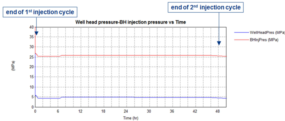
Figure 5b. Computed injection pressures after two days of injection by simulations using WI/CRI model
