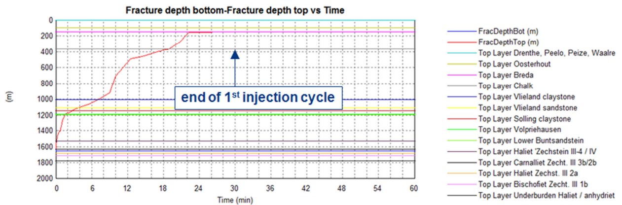
Figure 16. Results after 1 hour of injection of simulations using WI/CRI model. High injection rates, low modulus in top sands (0.1 GPa).
