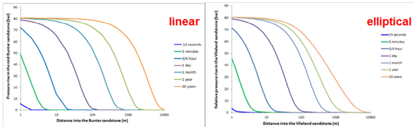
Figure 8. Pore pressure penetration in the Bunter sandstone
