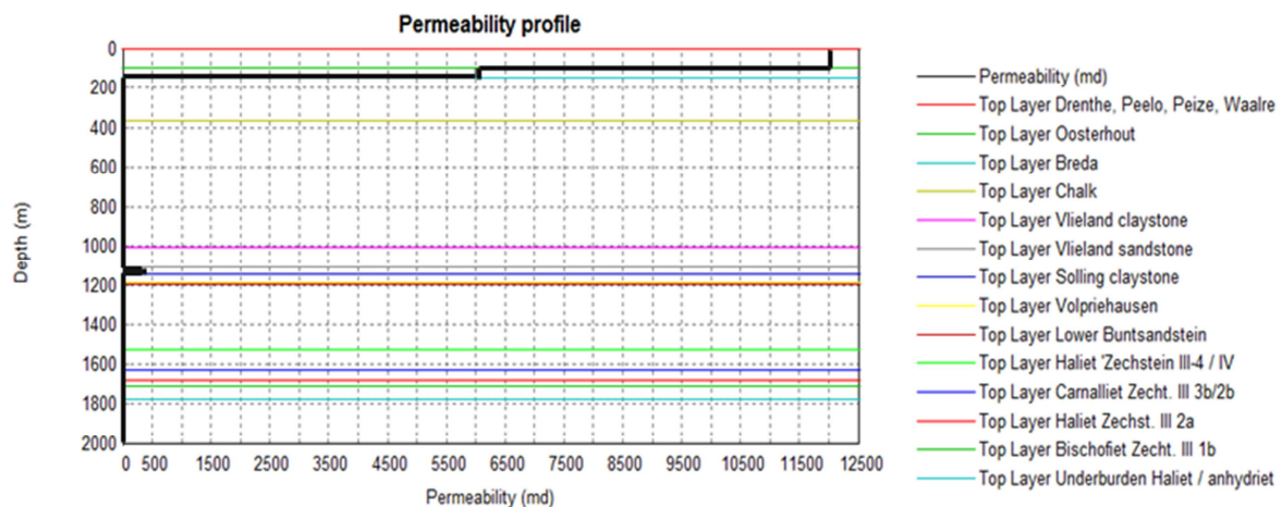
Figure 3. Permeability profile
