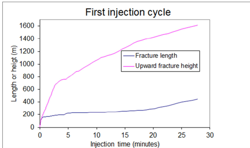
Figure 10b. Fracture growth during first 28 minutes of injection, simulations using BEM model, no stress contrasts between sands and clays.
