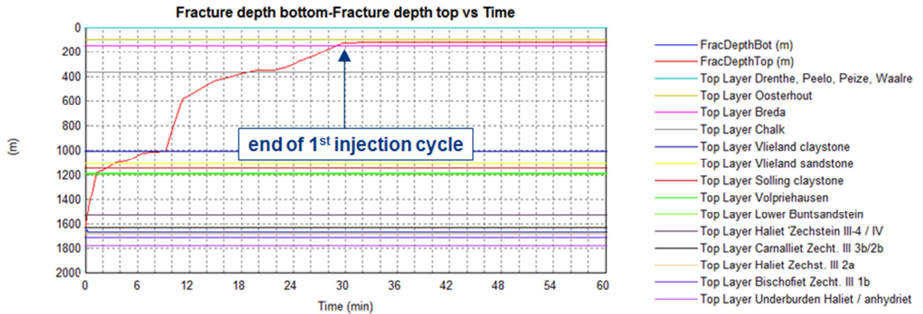
Figure 18. Results after 60 minutes of injection of simulations using WI/CRI model. For this case, all formations into which (some) brine leakage takes place had their permeabilities lowered by a factor 3.
