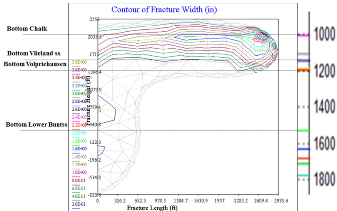
Figure 6a. Fracture geometry (plus mesh) after 30 minutes of injection, simulations using BEM model
