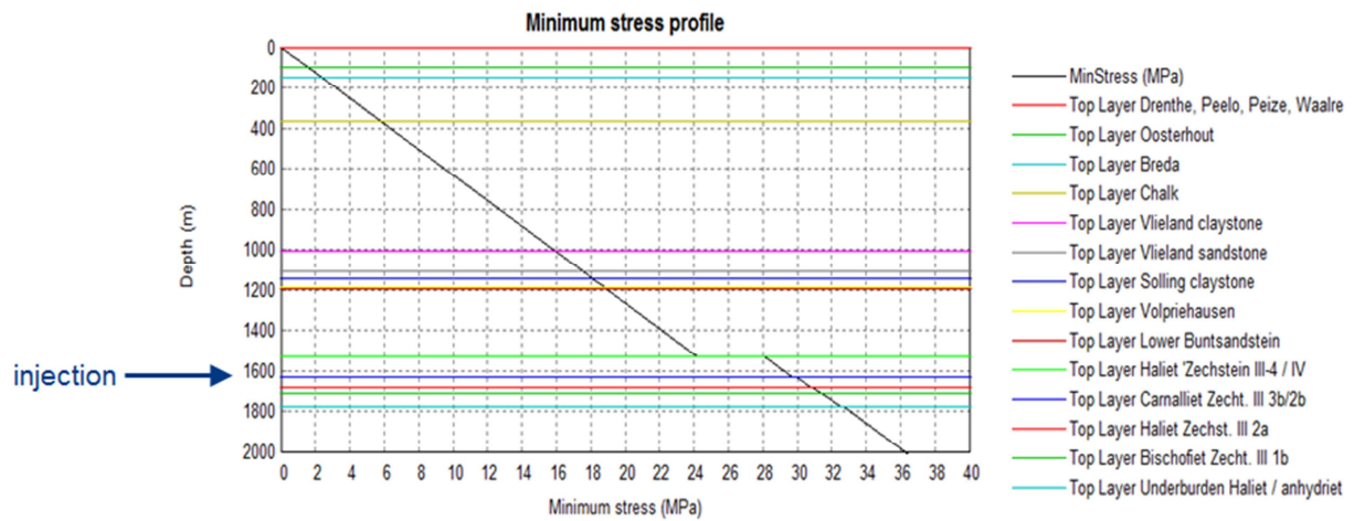
Figure 9. Zero stress contrasts between sands and clays in the overburden
