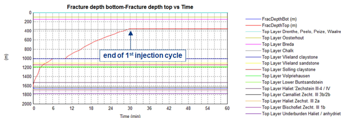
Figure 12. Results after one hour of injection of simulations using WI/CRI model. No stress contrasts between sands and clays.
