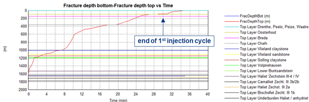
Figure 13. Results after 40 minutes of injection of simulations using WI/CRI model. High injection rates.
