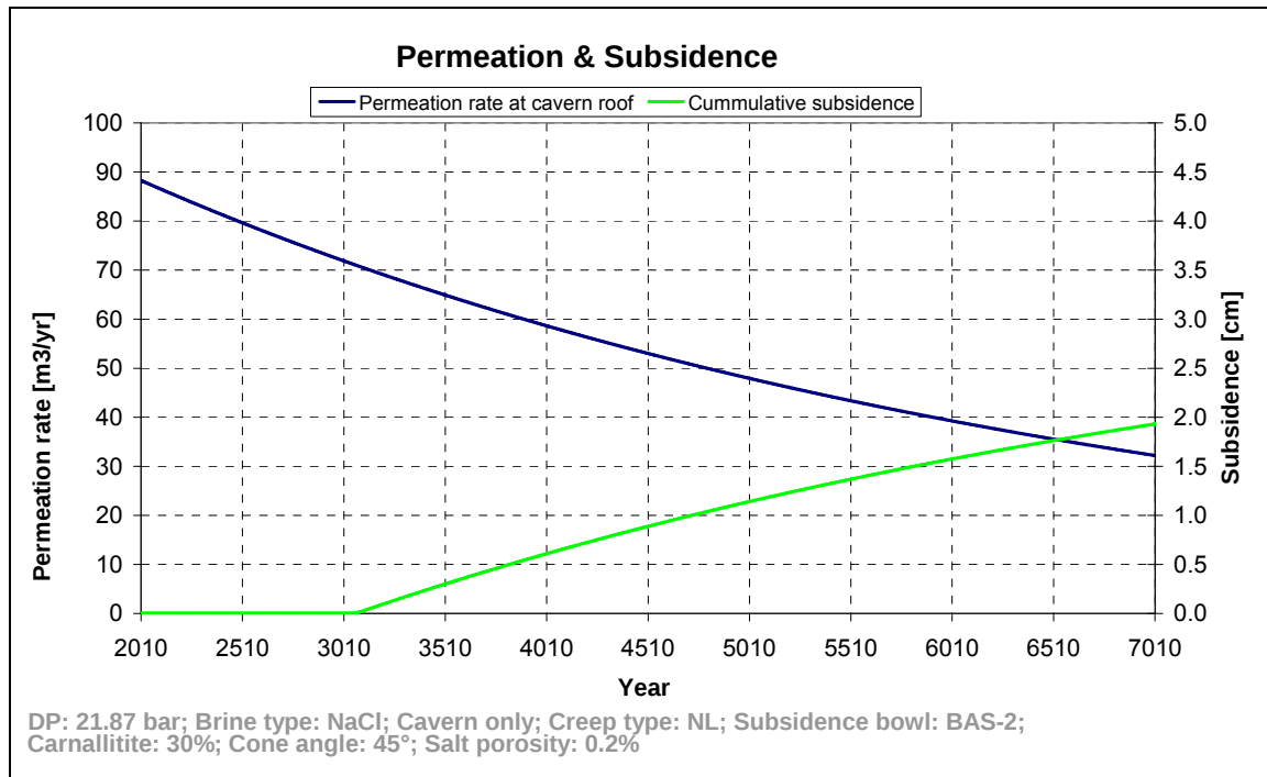
Figure 29 Sensitivity to subsidence bowl parameter.
