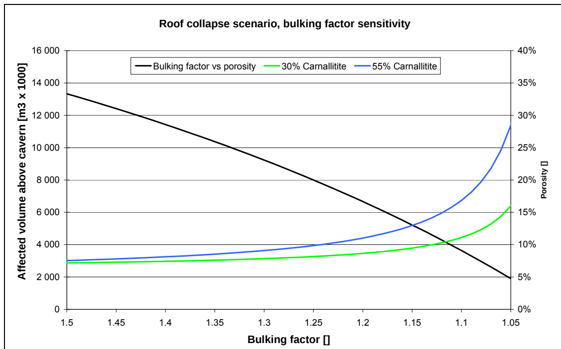
Figure 21 Sensitivity to bulking factor
