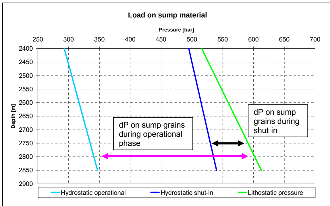
Figure 4 Loading of sump grains in operational and abandonment phase.
