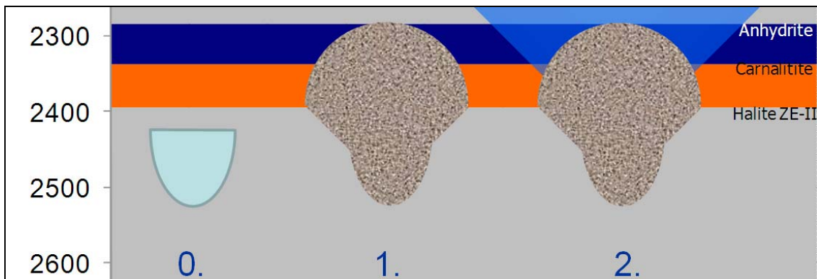
Figure 20 BAS-3 Impression of roof breakthrough scenario cavern development
