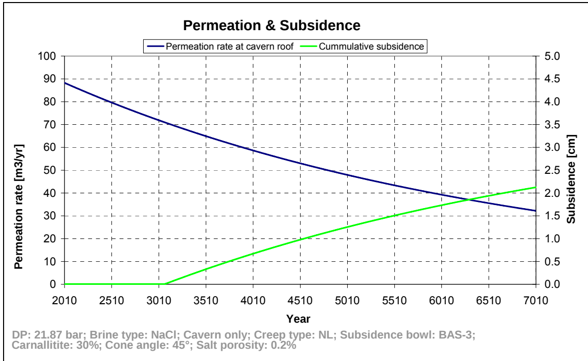
Figure 19 Base case permeation rate and subsidence over 5000 years.
