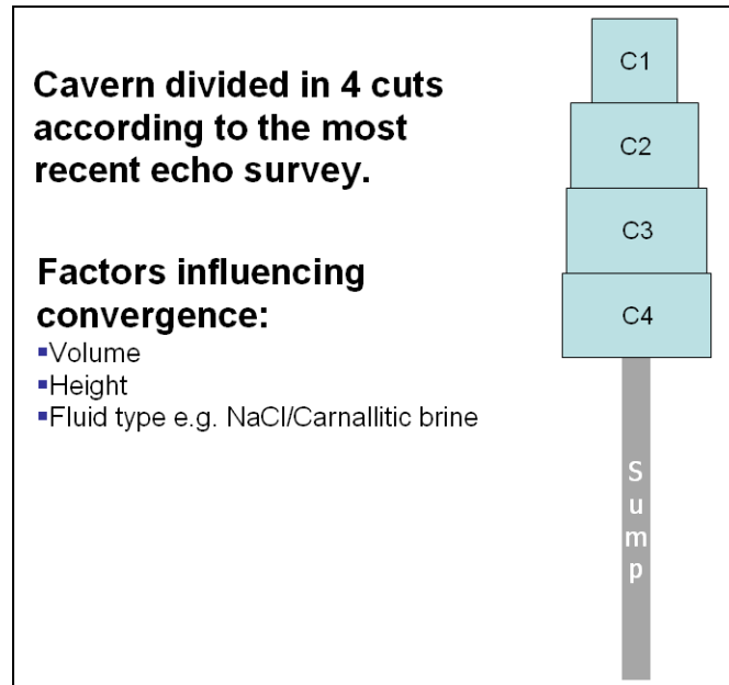
Figure 15 Model setup, partitioning into cuts according to last BAS-3 echo survey
