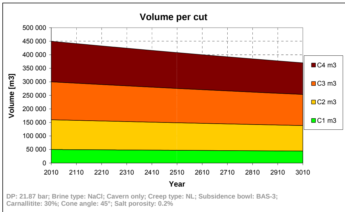
Figure 16 Base case volume development over the first 1000 years.
