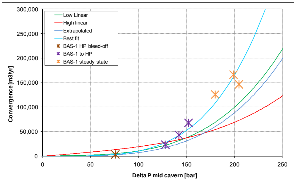
Figure 6 Convergence rate at a large range of pressure differentials.
