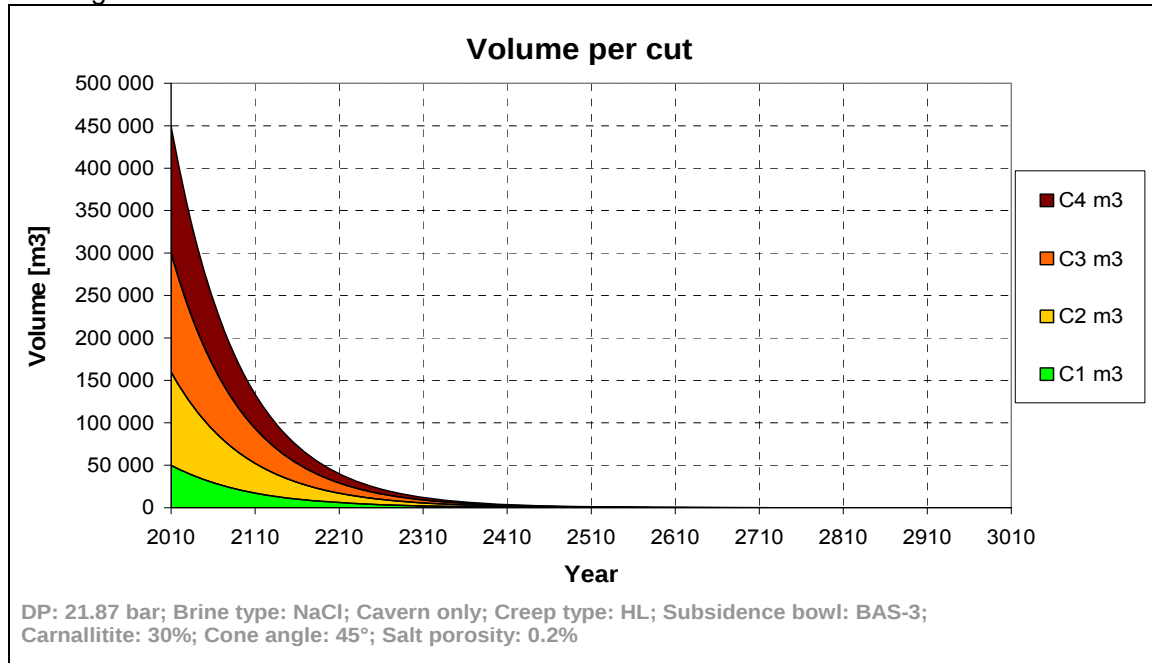
Figure 22 High linear variant volume development during the first 1000 years.
