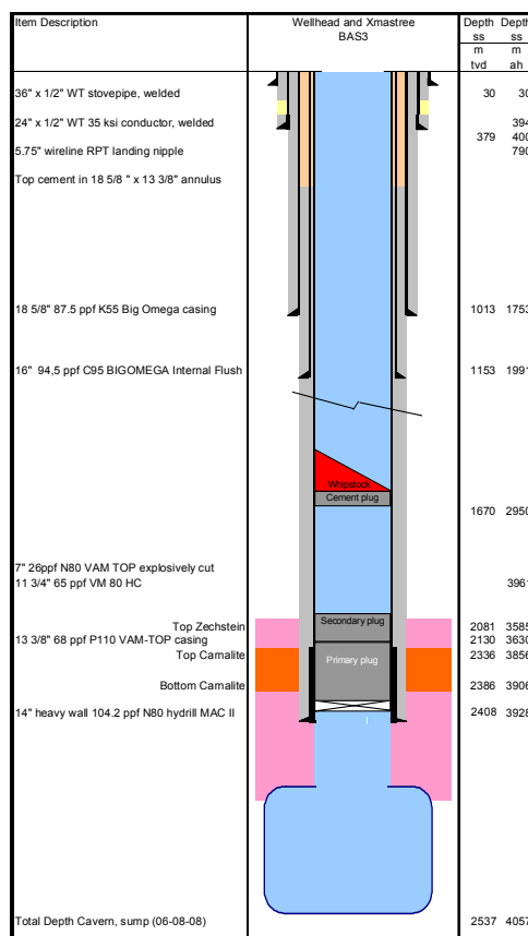
Figure 10 Sketch of the technical abandonment, including first preparations for a sidetrack
