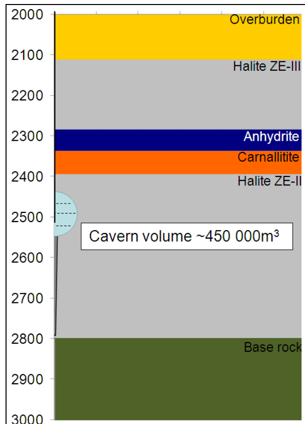
Figure 2 Geological cross section of BAS-3.
