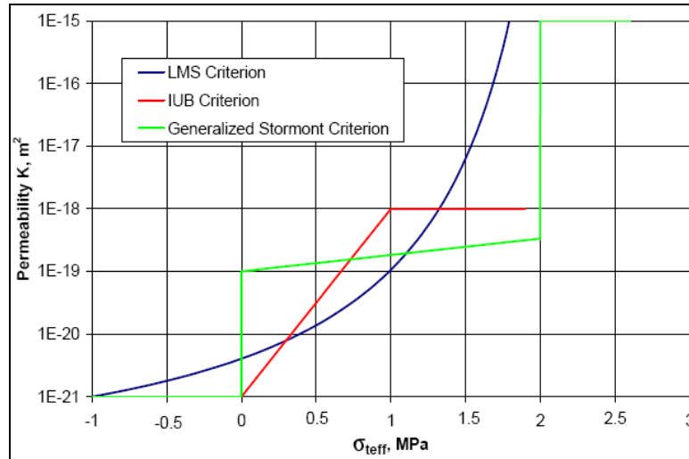
Figure 8 Various secondary permeability criteria. [ROKAHR 2002].
