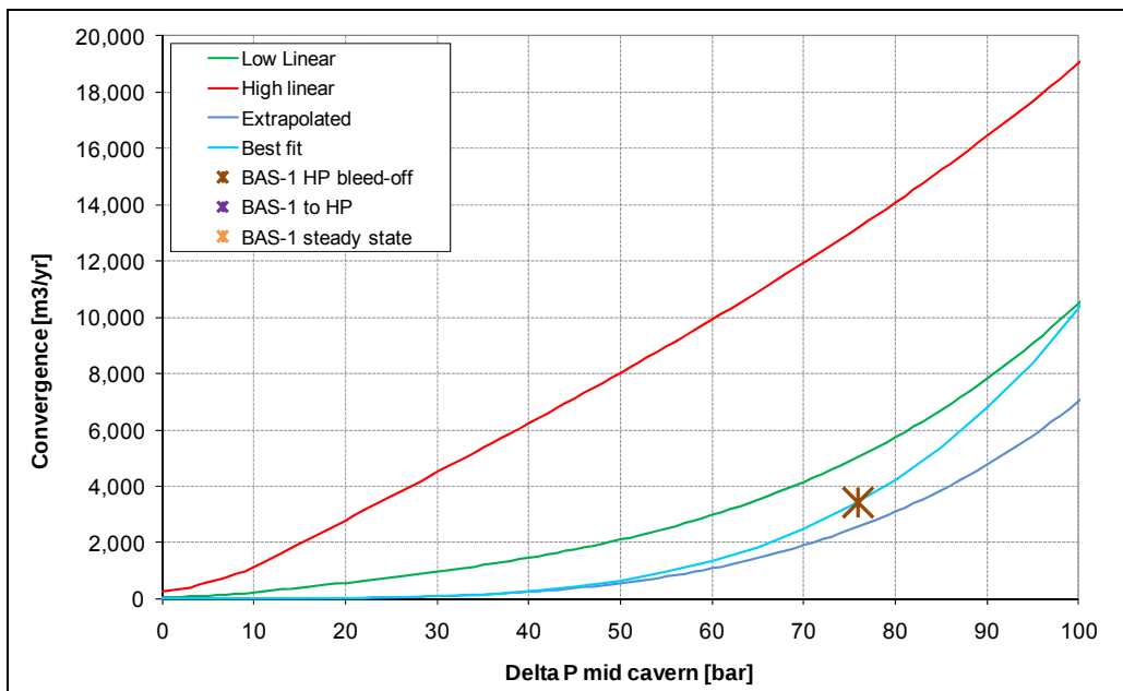
Figure 7 Convergence rate at low pressures differentials.
