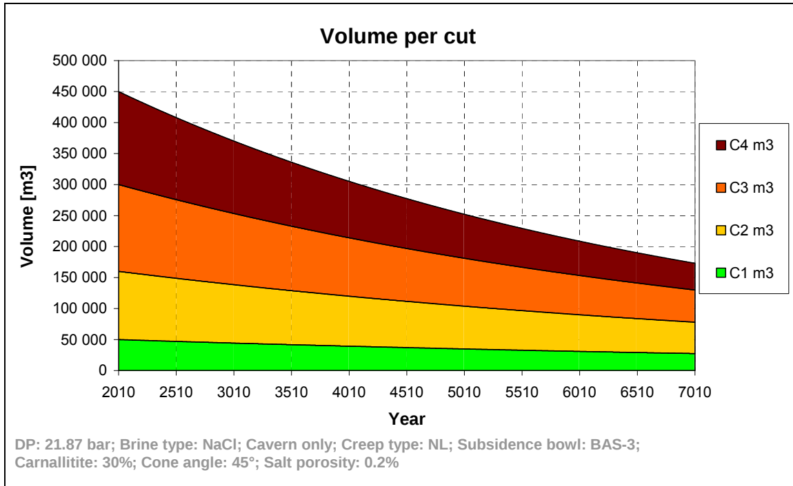
Figure 17 Base case volume development over 5000 years.
