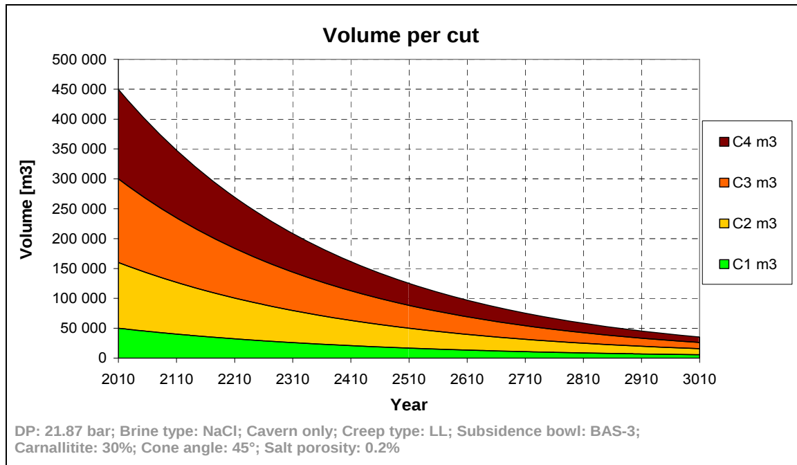
Figure 23 Low linear variant volume development during the first 1000 years.
