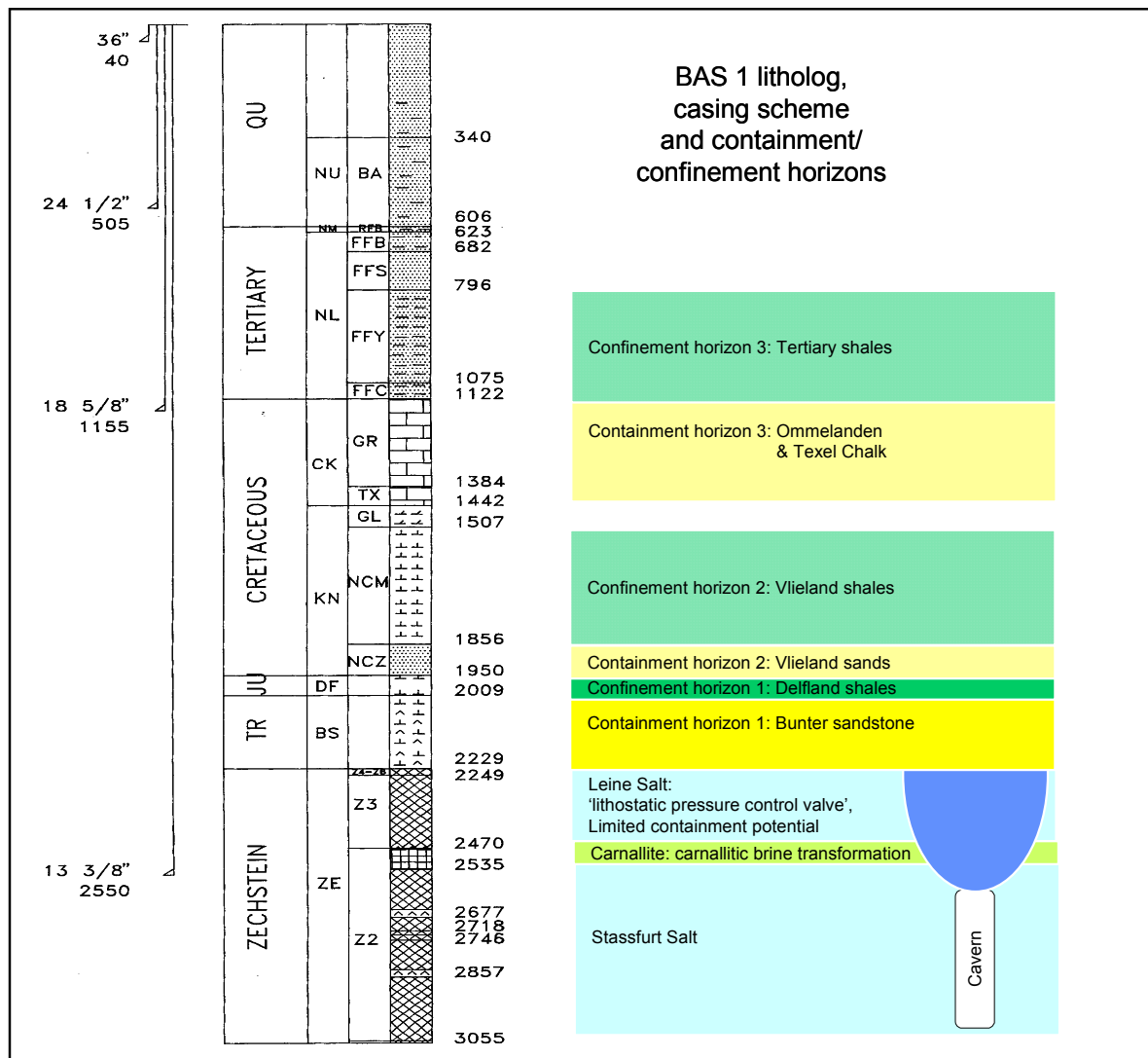
Figure 13 Overview of geological strata above BAS-1 showing containment and confinement horizons.
