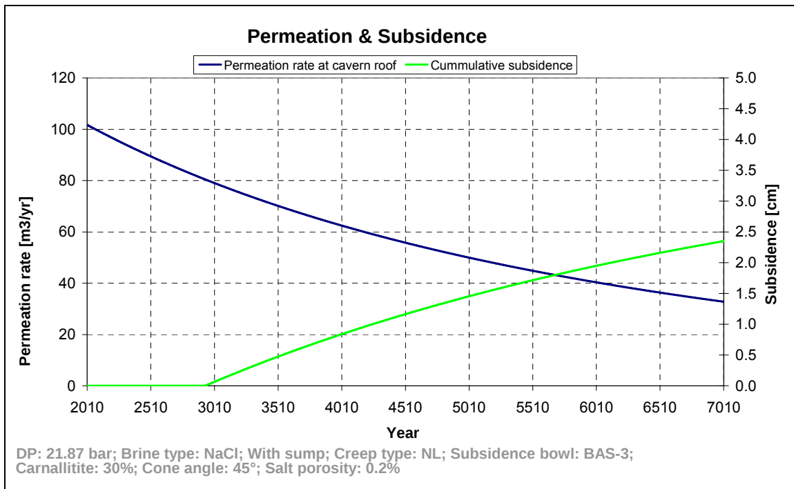
Figure 28 Sensitivity to sump permeation rate and subsidence.
