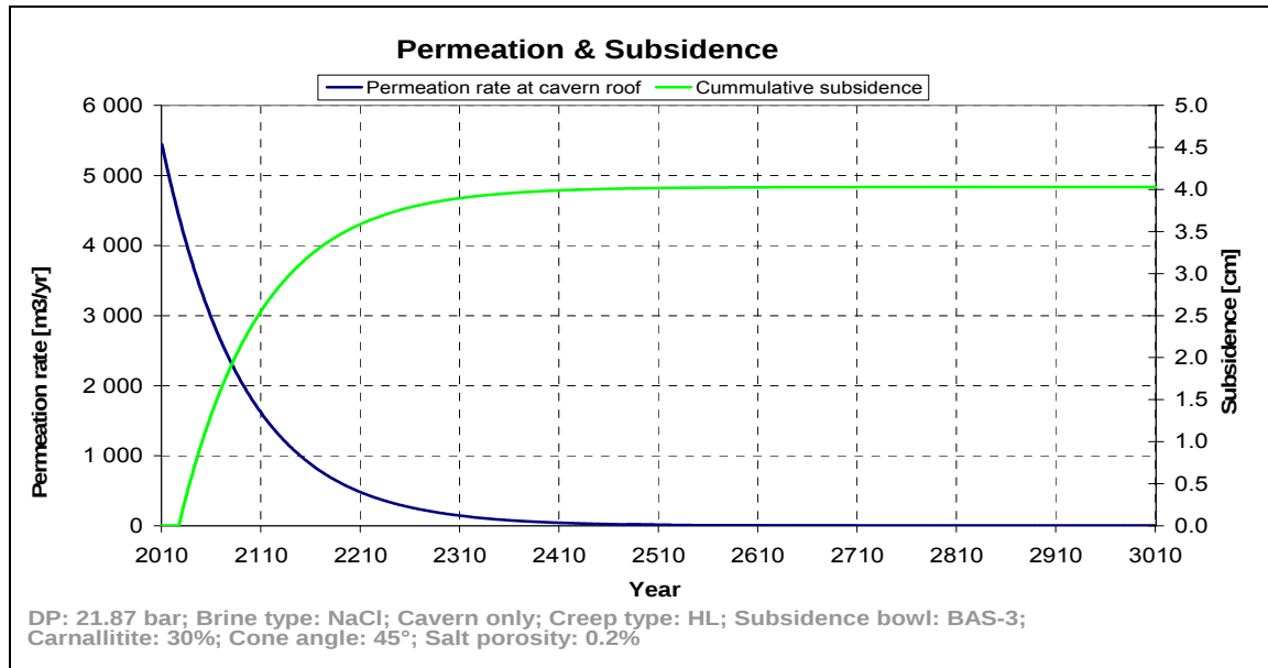
Figure 24 High linear variant permeation rate and subsidence over the first 1000 years, without taking a rebound effect into account.
