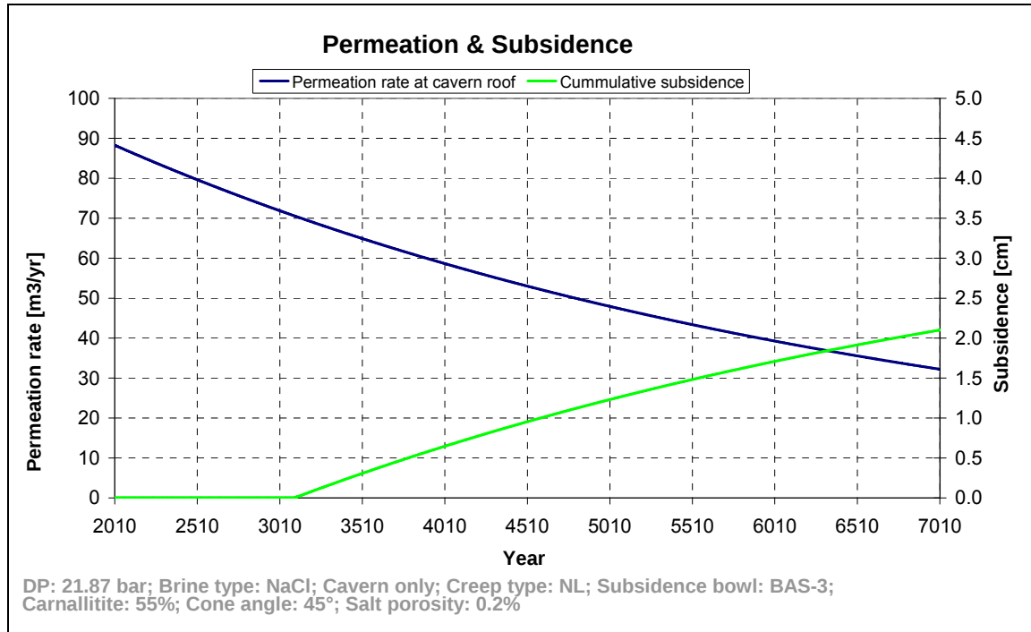
Figure 31 Sensitivity for 55% Carnallite variety.
