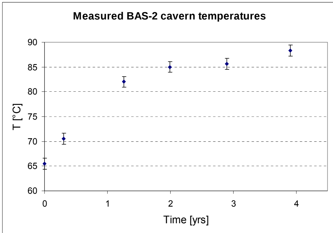
Figure 5 Temperature build-up BAS-2 cavern after shut-in in October 2004.
