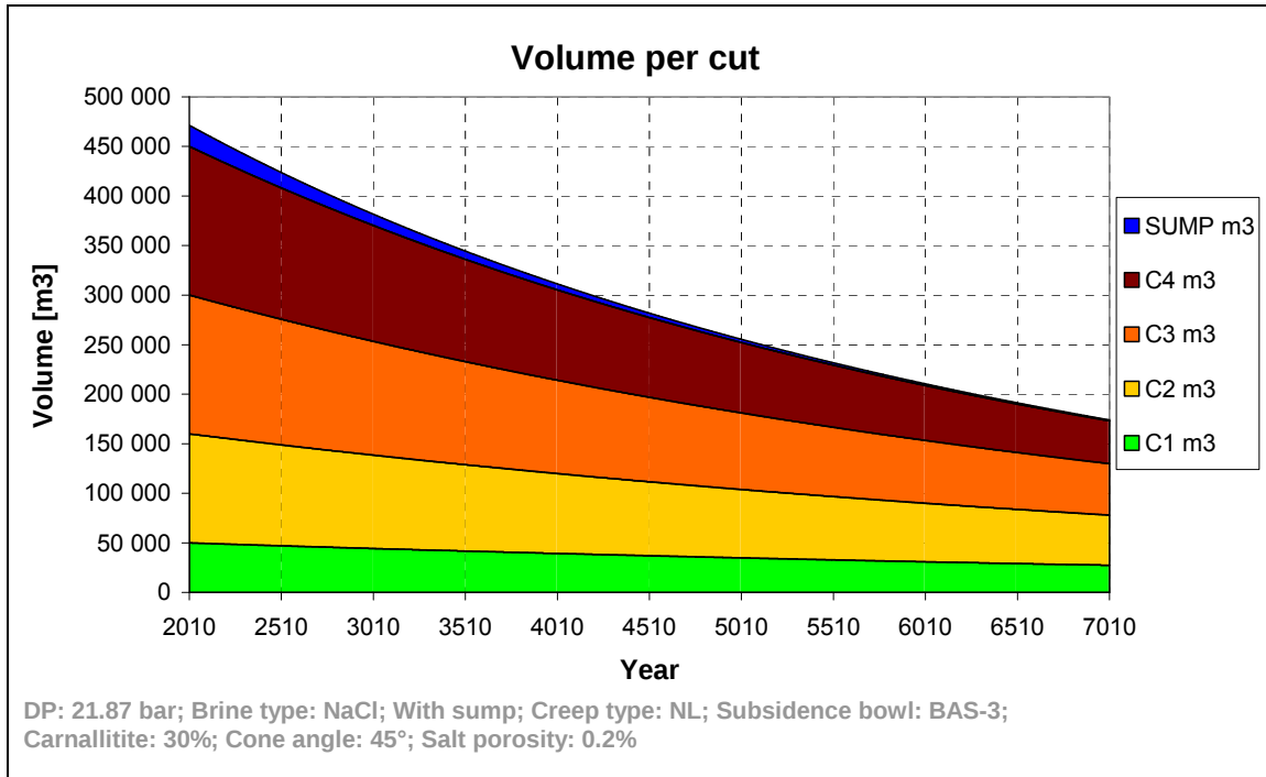
Figure 27 Sensitivity to sump volume development.
