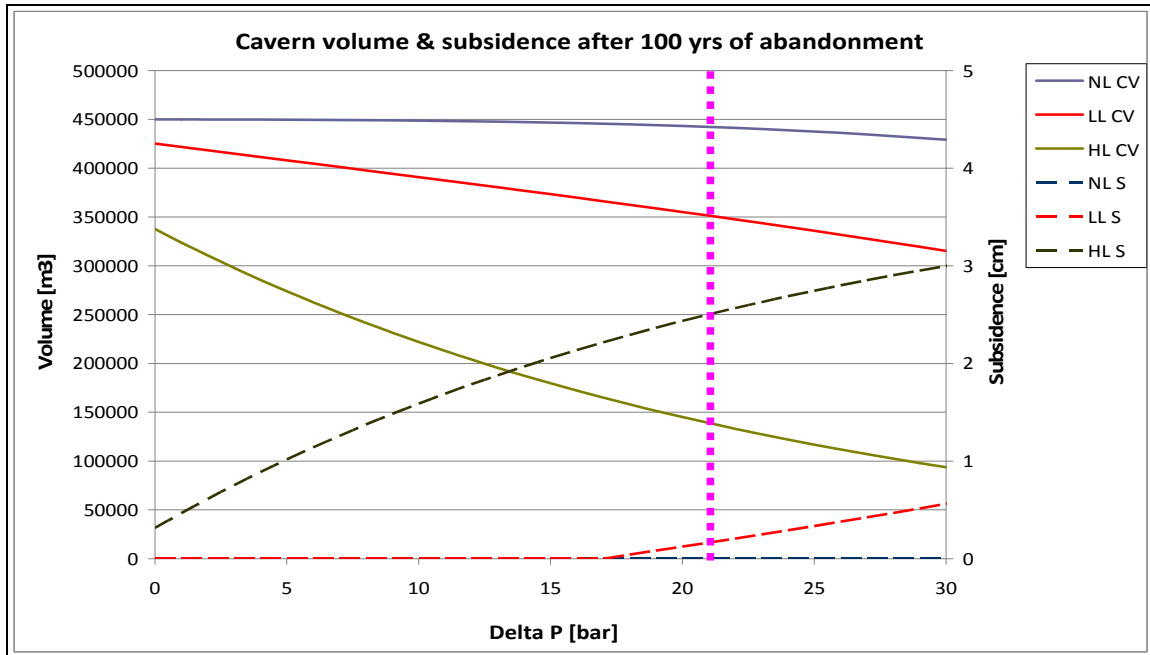
Figure 26 Cavern volume (CV) and subsidence(S) after 100yrs for various pressure differences (lithostatic minus cavern pressure) at the 13 3/8" shoe and the various creep variants for the BAS-3 cavern volume, the continuous lines depict the cavern volume, the dashed lines the subsidence and the pink dotted line the pressure difference used in the base case.
