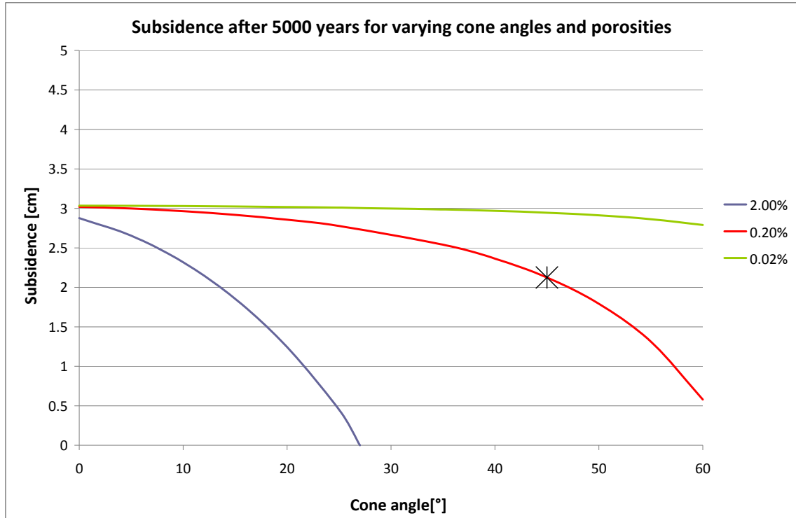
Figure 30 Subsidence sensitivity for storage capacity in the salt as a function of various permeation cone angles and porosities after 5000 years; the base case is marked with an asterisk.
