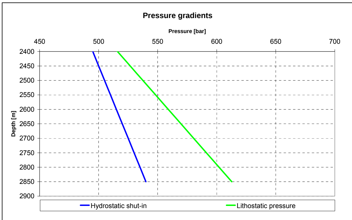
Figure 9 Expected pressure gradients 5 year after shut-in.
