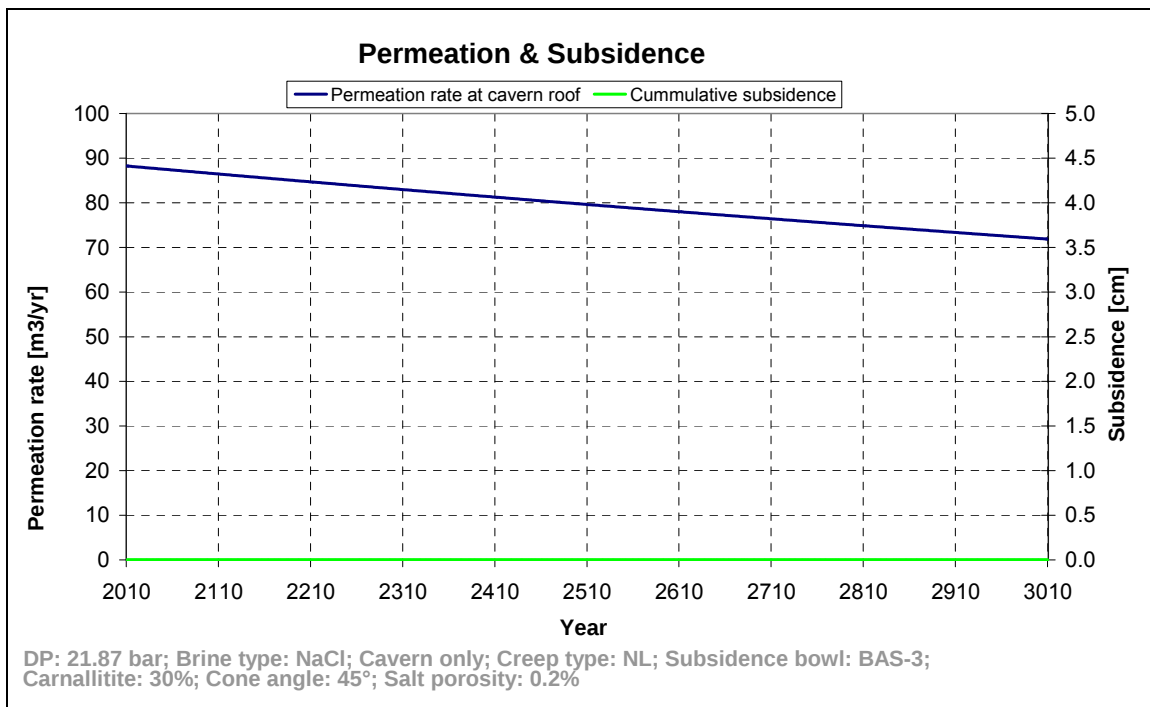
Figure 18 Base case permeation rate and subsidence over the first 1000 years.
