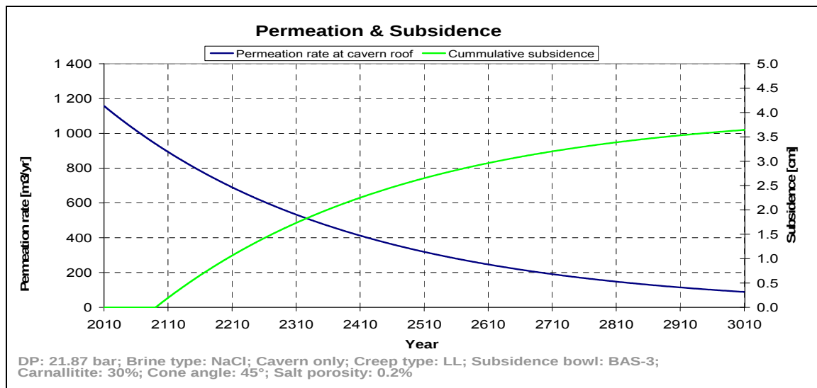
Figure 25 Low linear variant permeation rate and subsidence over the first 1000 years, without taking a rebound effect into account.
