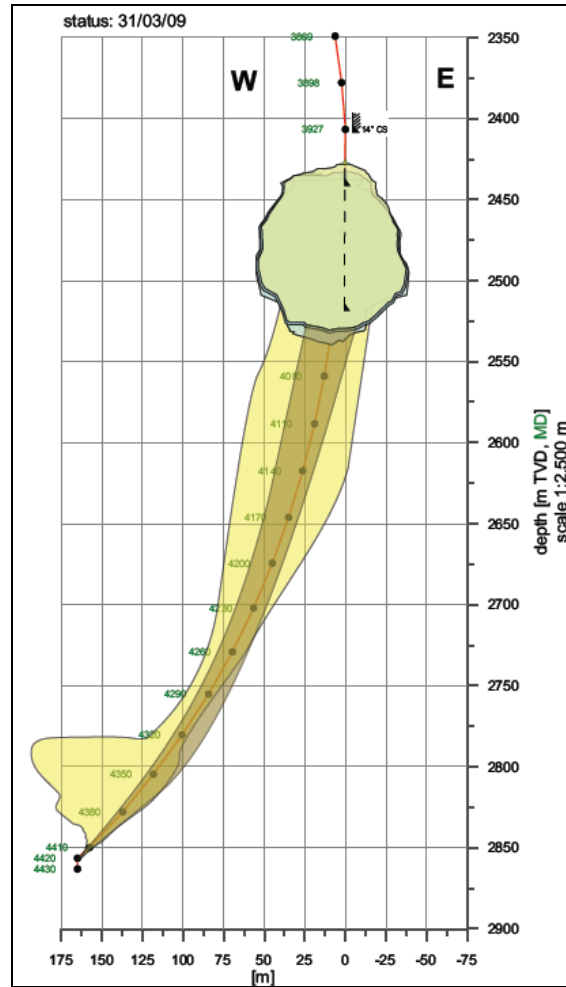
Figure 3 Impression of the BAS-3 cavern and sump tail shape [Fischer, 2010].
