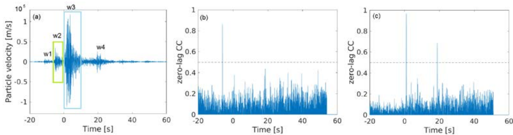
Fig. 13: (a) Winschoten event with the 4 subevents labeled: W1, W2, W3 and W4. (b) and (c) show matching results of W2 and W3, respectively, with the 80 seconds recording as shown in (a). A matching is obtained when a cross-correlation coefficient is obtained larger than 0.5.
