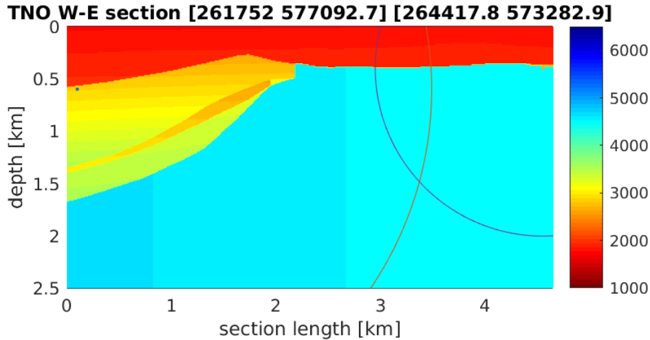
Fig. 10: Section through Velmod-3 (Dalfsen et al., 2006) between stations G52 and G57 of the KNMI network. The colour map shows P-wave velocities. Blue correspond to mostly halite deposited in Perm, yellow to green corresponds to chalk from the Cretaceous and red corresponds to mostly unconsolidated sediments from the Paleogene and Neogene. The red and blue line show P-S delay isochrones for geophones G524 and G574, respectively. The intersection of the two lines is an estimate of the hypocentre.
