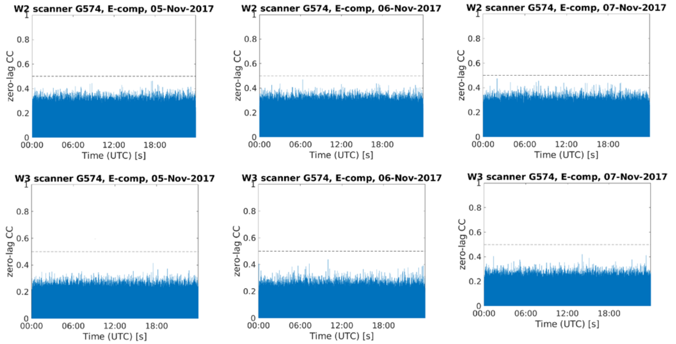
Fig. B.1: Template matching from day of year 309 to 311, with template W2 (upper panels) and W3 (lower panels). The template events have been defined in Fig. 13(a).
