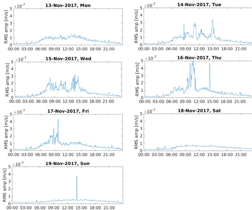
Fig. 15: root-mean-square (RMS) amplitudes of the vertical component at station G57 for one week of continuous data bandpass filtered between 5 and 40 Hz. The RMS amplitude is computed over a sliding widow of 300 seconds, with a 50 percent overlap.
