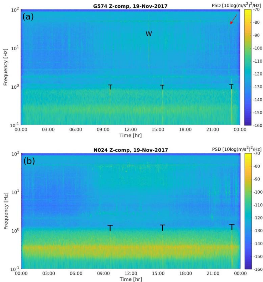
Fig. 12: Spectrograms for vertical-component recording of geophone (a) G574 and (b) N024. Geophone G574 is located on top of the Heiligerlee dome, whereas N024 is located near the village of Norg, 38 km WSW of station G574. The Winschoten event is denoted with 'W', 3 teleseismic events are denoted with 'T'. The red arrow highlights an event with unknown origin.
