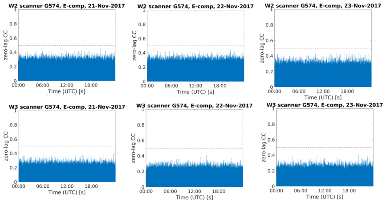
Fig. B.6: Template matching from day of year 325 to 327
