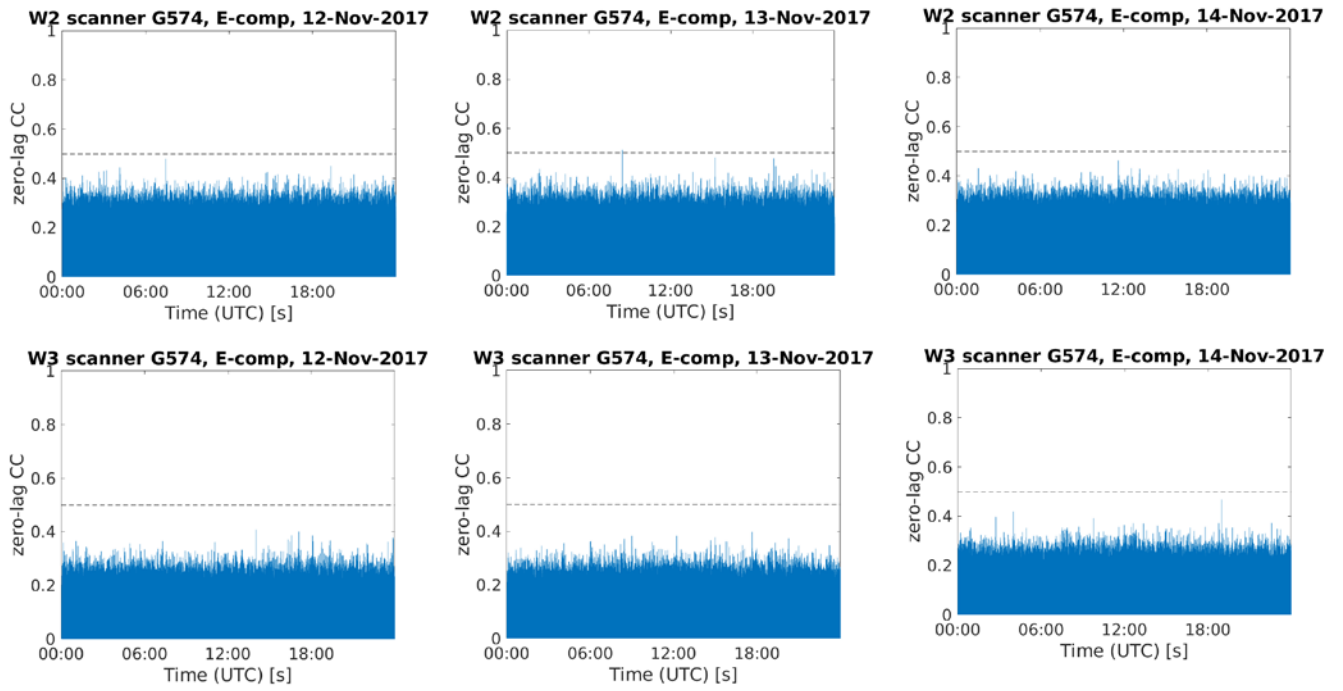
Fig. B.3: Template matching from day of year 316 to 318
