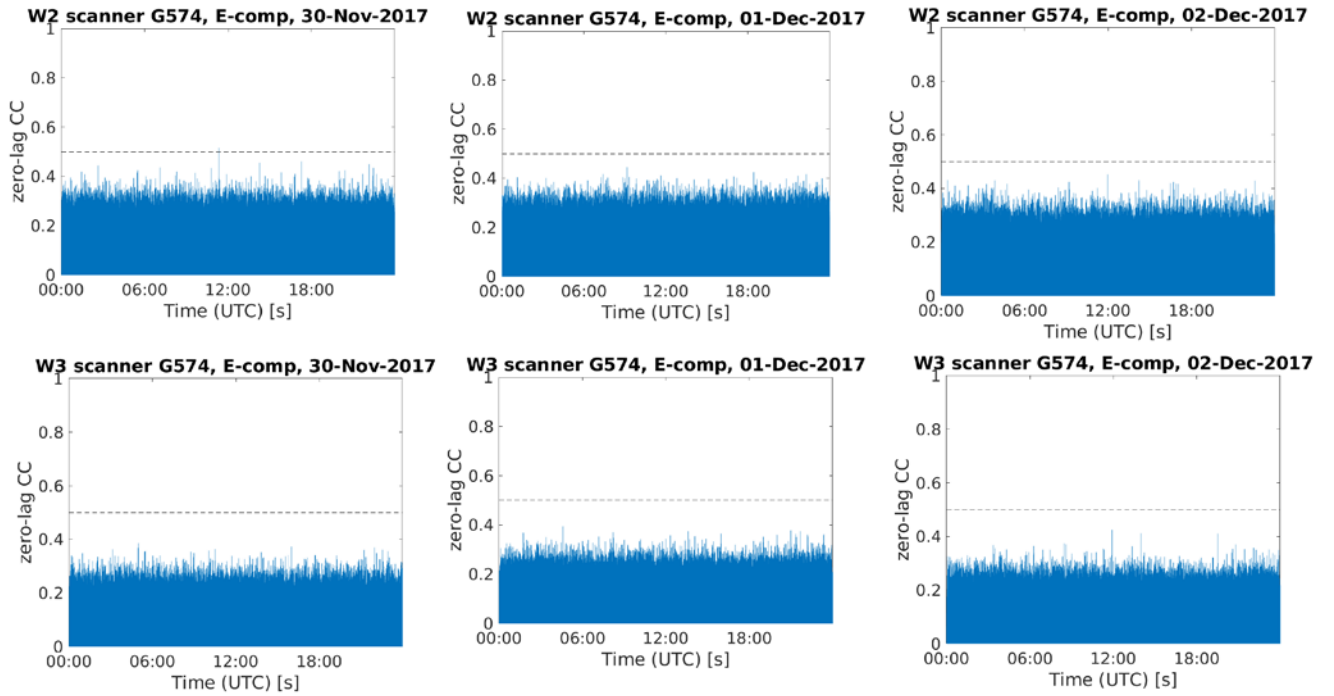
Fig. B.9: Template matching from day of year 334 to 336
