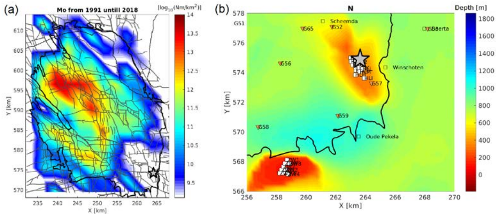
Fig. 2: (a) Distribution of the total seismic moment release (colour map) over the Groningen gas field (black solid line) between 1991 and January 2018, and the SeisComp3 source location (grey star) for the 19-11-2017 event. Faults at reservoir level are denoted by grey lines. (b) Area of interest around Winschoten, with the source location (grey star) and KNMI seismic stations (orange triangles) indicated. The colour map shows the depth of the North Sea Group, with two highs (red) where salt domes exist. White squares denote salt caverns (Appendix A) and the black solid line shows the south-eastern edge of the Groningen gas field.
