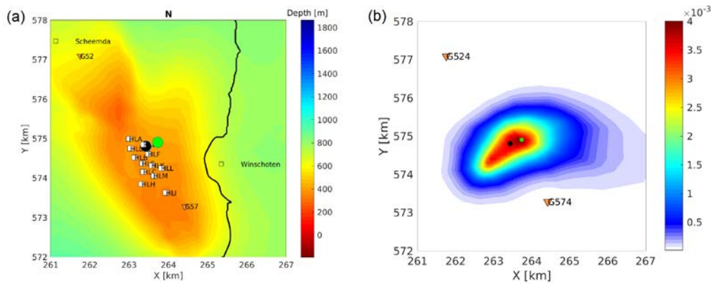
Fig. 9: (a) The Heiligerlee salt dome (warm colours), locations of caverns in it (white squares) and both the initial location (black dot, SeisComp3) and the updated location (green dot, EDT). (b) shows the probability density function for the EDT method.
