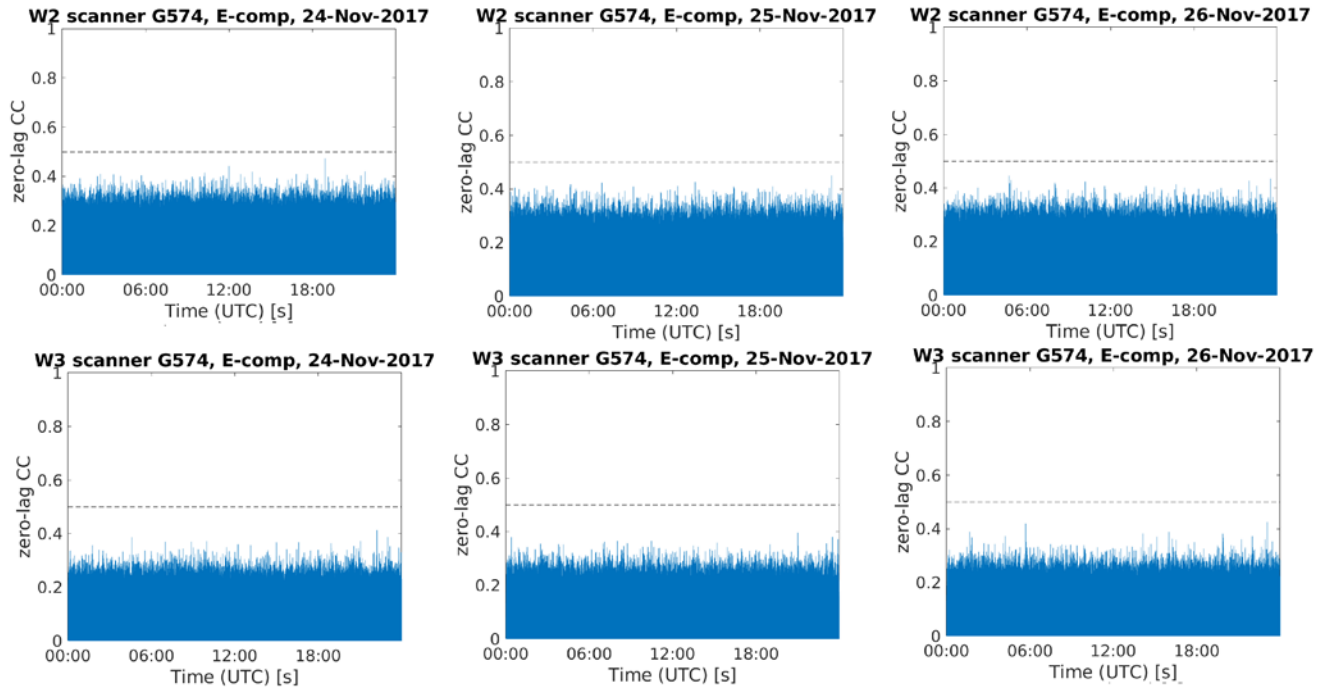
Fig. B.7: Template matching from day of year 328 to 330
