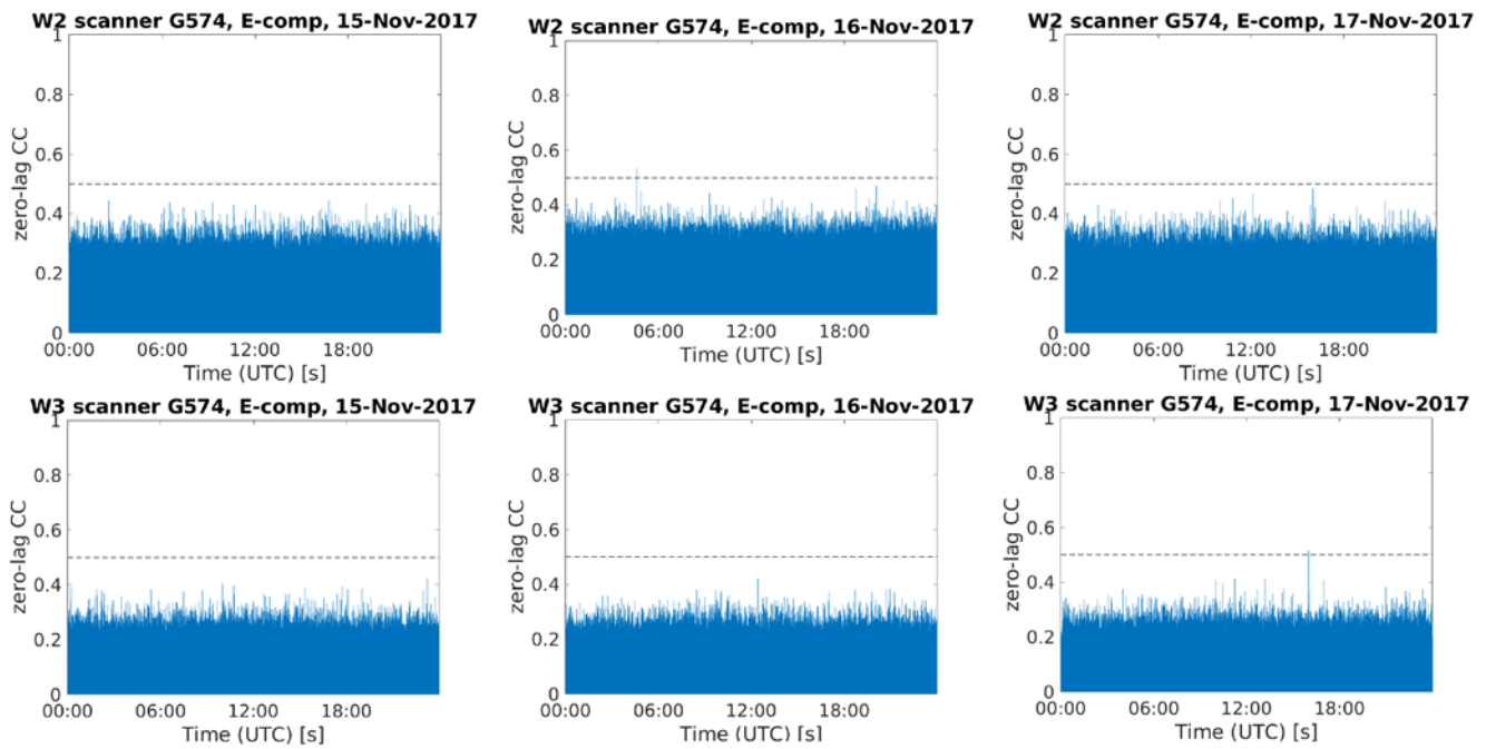
Fig. B.4: Template matching from day of year 319 to 321
