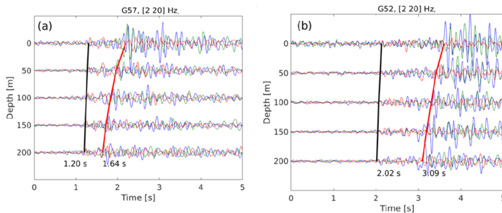
Fig. 5: (a) 3-component response at 5 depth levels in boreholes (a) G57 and (b) G52. The red, blue and green seismograms denote the vertical, radial and transverse particle velocity recordings. Thick black and red lines denote depth-consistent picks of the first P- and S-wave onset, respectively.
