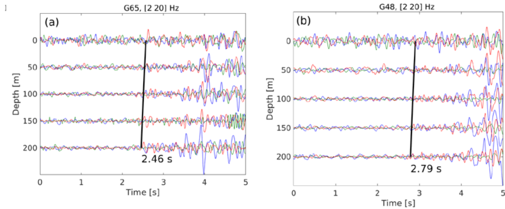
Fig. 6 (a) 3-component response at 5 depth levels in boreholes (a) G65 and (b) G48. The red, blue and green seismograms denote the vertical, radial and transverse particle velocity recordings. Thick black lines denote depth-consistent picks of the first P-wave onset. Geophone G653 (depth level 150 m) has malfunctioning horizontal components.
