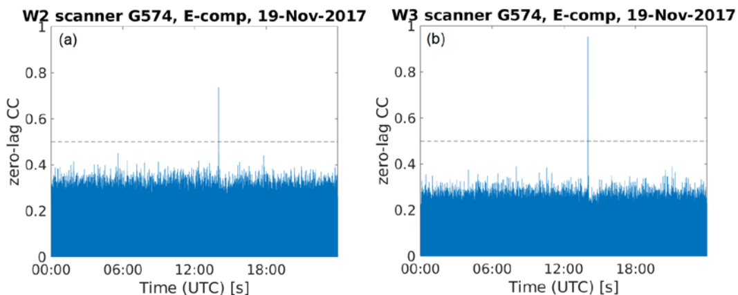
Fig. 14: Results of scanning through 1 day of continuous data with templates (a) W2 and (b) W3 (templates have been defined in Fig. 12(a)). A zero-lag cross-correlation (CC) coefficient of more than 0.5 means that likely a similar event was recorded.
