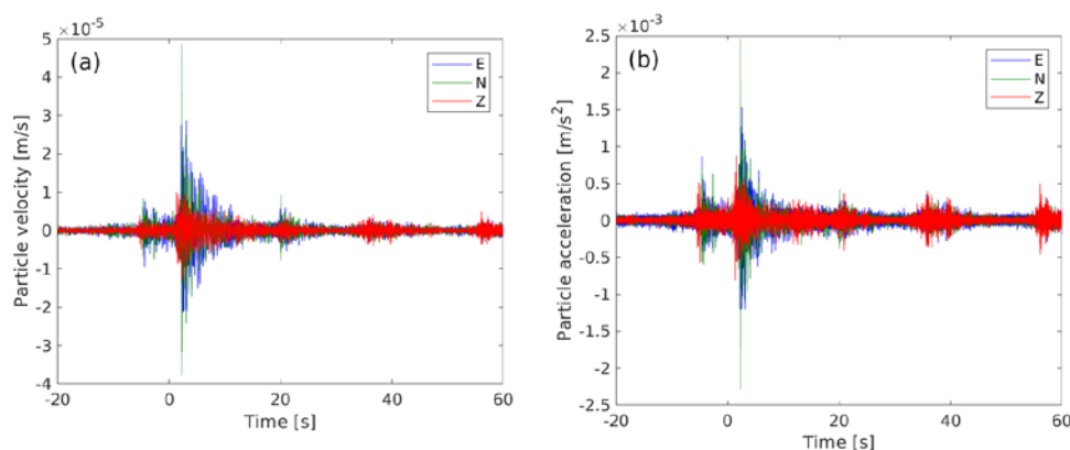
Fig. 1: 3-component recordings at sensor G570, expressed in (a) particle velocity and (b) particle acceleration. E, N and Z denote east, north and vertical movements, respectively. The zero time corresponds to the SeisComp3 earthquake origin time of the main event: 19-11-2017 14:00:48 UTC (15:00:48 local time).
