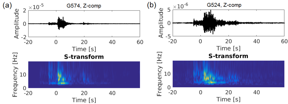
Fig. 4: Recording of the Winschoten 19-11-2017 events at the two nearest sensors at 200 m depth: (a) G574 and (b) G524. The upper panels show registrations in the time domain, the lower ones show the recordings mapped to the time-frequency domain using the S-transform.
