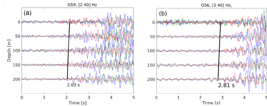
Fig. 7: (a) 3-component response at 5 depth levels in boreholes (a) G59 and (b) G56. The red, blue and green seismograms denote the vertical, radial and transverse particle velocity recordings. Thick black lines denote depth-consistent picks of the first P-wave onset.
