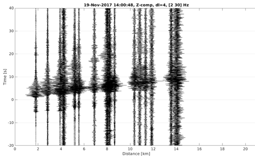
Fig.3: Event gather of vertical-component particle velocity recordings at 200 m depth, frequency band-pass filtered between 2 and 30 Hz.
