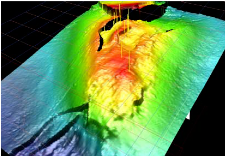
Figure 5: 3D perspective view of the base Tertiary. The horizon is situated on top of the dome close to the caprock. Hence, the picture shows the shape of the top of the dome. The yellow lines represent the well trajectories above the base Tertiary. Obvious are the faulted areas, caused by salt dissolution, at the top and next to the dome.
