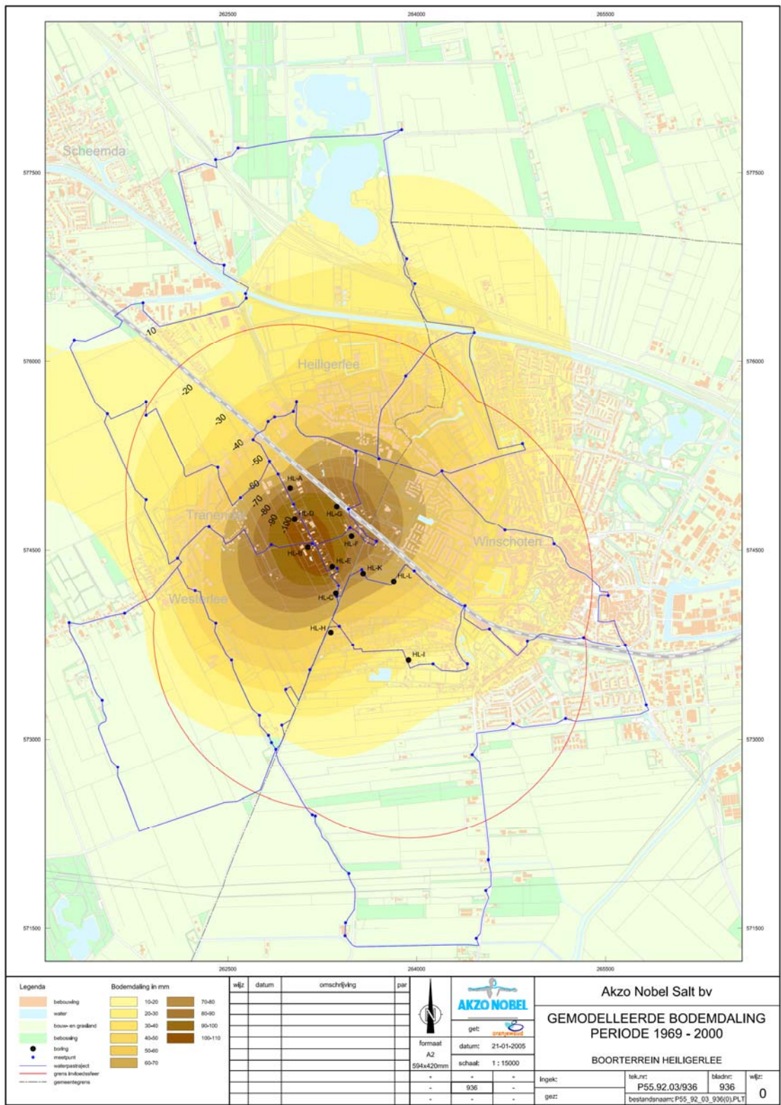
Figure 3: Modelled soil subsidence map, period 1969-2000, assuming the subsidence modelling is based on data collected at the blue water pressure measurement points.
