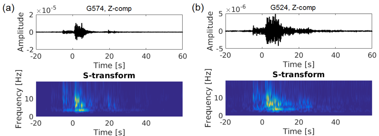
Figure 2: Figure from the KNMI report. Recording of the Winschoten 19-11-2017 events at the two nearest seismic sensors, namely G574 (a) and G524 (b). On top panels are the registration in the time domain, on underlying panels in the time-frequency domain.
