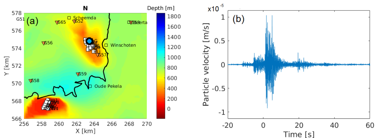
Figure 1: Figure from the KNMI report (a) Area around Winschoten showing the depth of the North Sea group sediments (colour scale), the border of the Groningen gas field (black line), KNMI seismic stations (orange triangles), salt caverns (white squares) and the Seiscomp3 location (blue dot). (b) Vertical component registration at sensor G574 (the 200 m depth level of station G57). The no-stop time corresponds to 14:00:48 UTC (15:00:48 local time) on 19/11/2017.
