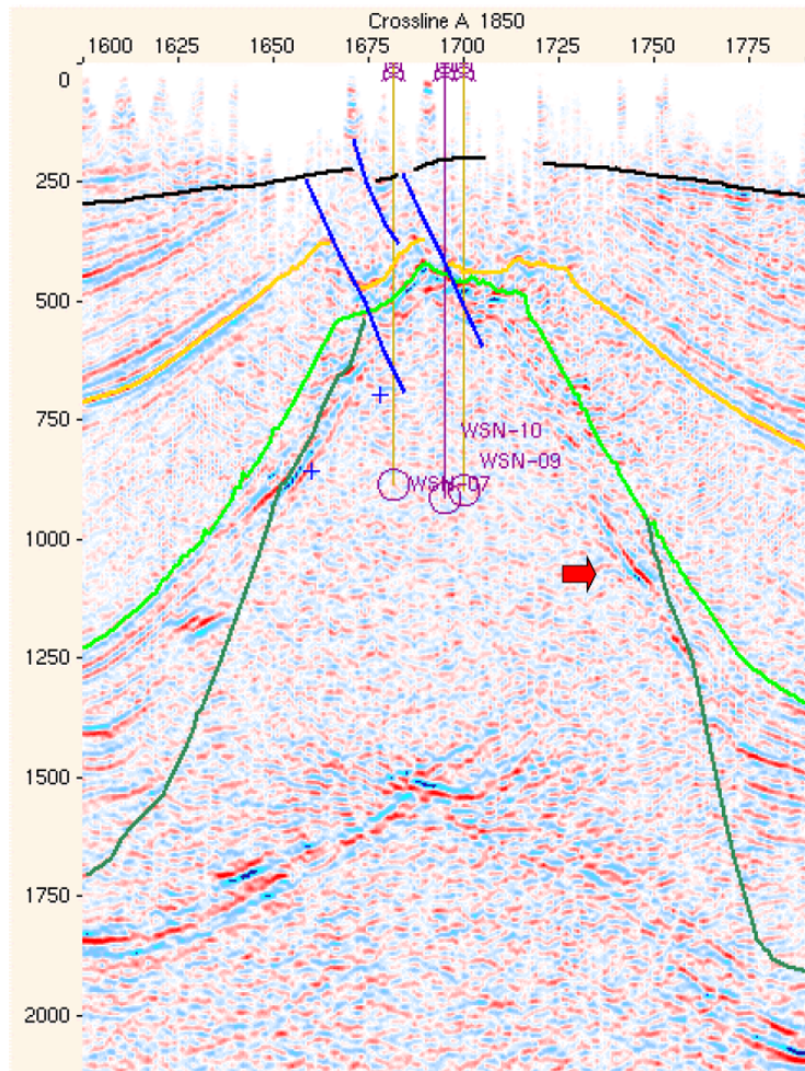
Figure 4: Example of an E-W seismic line from the Blijham-Groningen 3D survey. Three wells are projected on this line. The data hiatuses in the uppermost part of the section are due to data acquisition problems. The top of the dome is imaged by the dark green line. The red arrow indicates the position of an anhydrite floater or a caprock relict.
