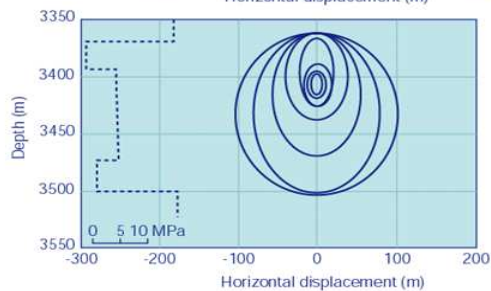
Figure 3: Comparison of WI/CRI fracture model with TERRAFRAC (BEM) and MFRAC for NAM offshore MHF.
