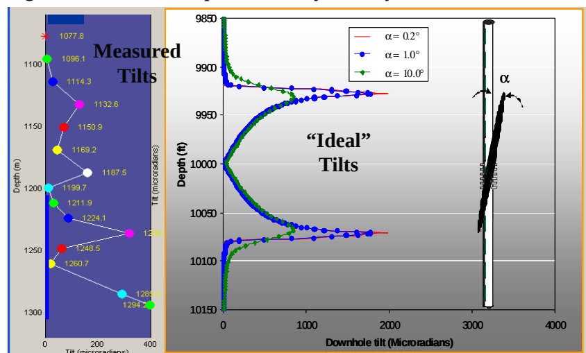
Fig. 12. Oman water disposal well: Example of tiltmeter data
