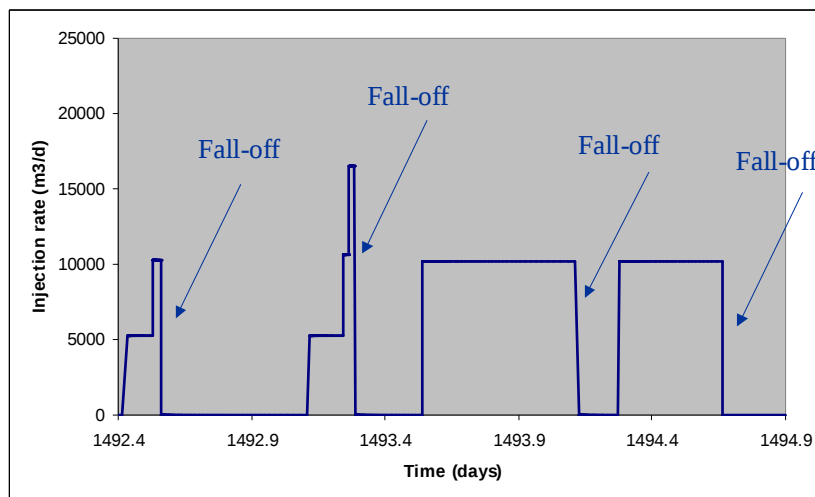
Fig. 11. Oman water disposal well: Injection cycles of tiltmeter test
