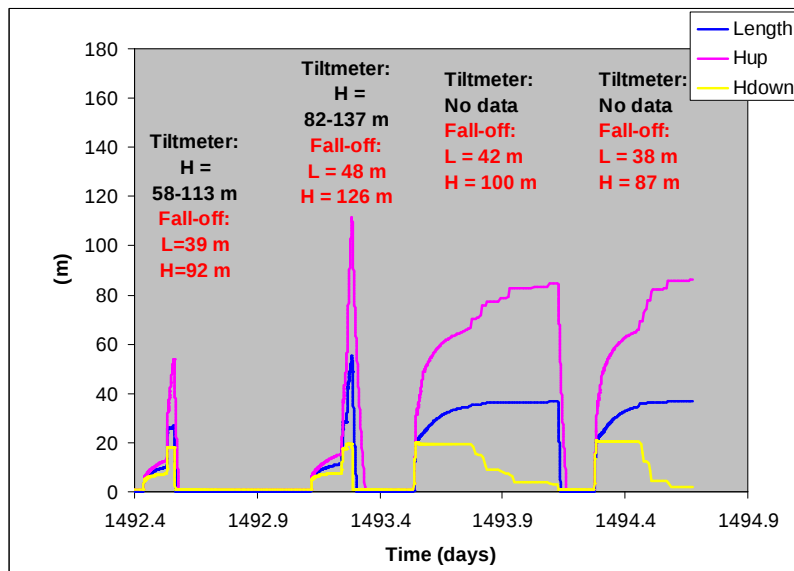
Fig. 14. Oman water disposal well: Summary of tiltmeter test results. Colored curves represent computed results: Length (L), Hup (=upward fracture height), and Hdown (downwards fracture height). H = \text{total fracture height} = \text{Hup} + \text{Hdown} .
