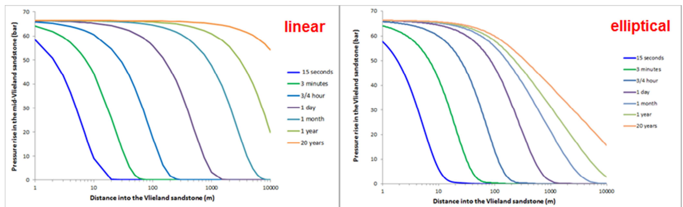
Figure 7. Pore pressure penetration in the Vlieland sandstone
