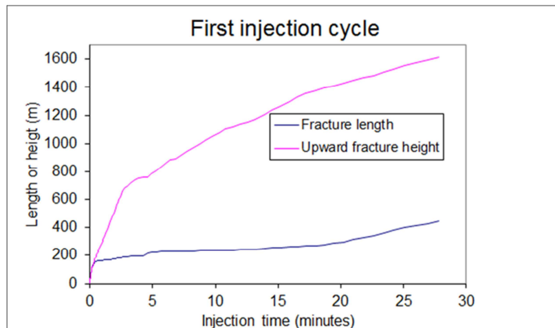
Figure 10b. Fracture growth during first 28 minutes of injection, simulations using BEM model, no stress contrasts between sands and clays.
