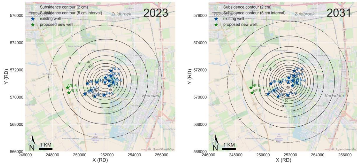
Figure 7-2 Subsidence forecast (in cm) for 2023 (left) and 2031 (right) based on production scenario 1 using the rigid basement parameters from the global minimum that resulted in the largest modelling error, see Appendix D. 2031 is the year when subsidence at a benchmark location reached the maximum permitted 65 cm.
