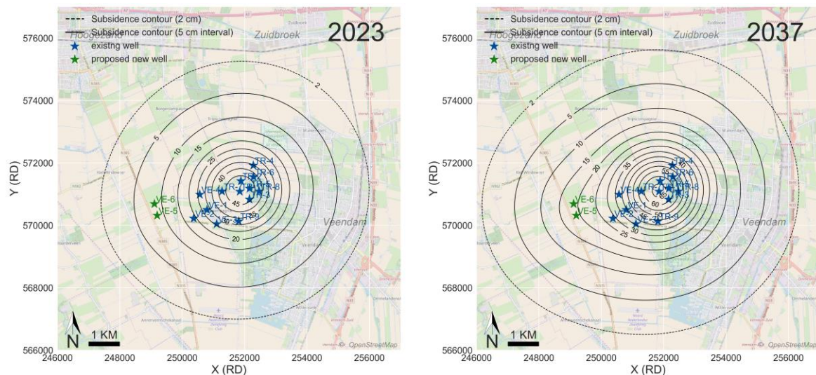
Figure 7-3 Subsidence forecast (in cm) for 2023 (left) and 2037 (right) based on production scenario 2 using the alternative rigid basement parameters. As a result of applying the alternative parameters to scenario 2 the maximum permitted subsidence at a benchmark location is reached in 2037, one year later than in the forecast reported in Chapter 3.
