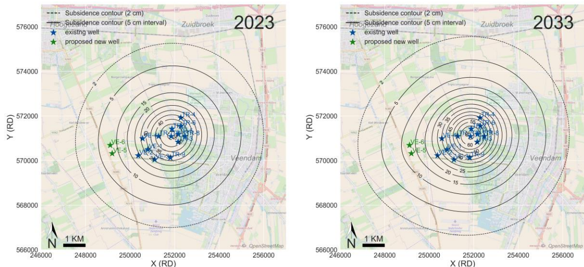
Figure 3-4 Subsidence forecast (in cm) for 2023 (left) and 2033 (right) based on production scenario 3.
