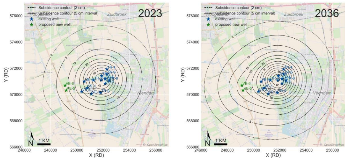
Figure 3-3 Subsidence forecast (in cm) for 2023 (left) and 2036 (right) based on production scenario 2.
