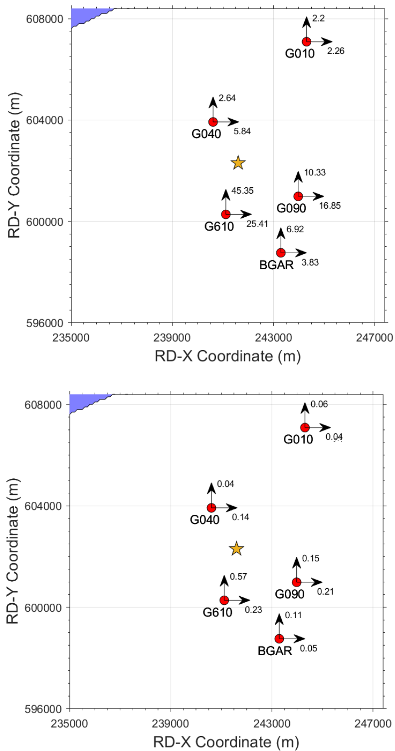
Figure 3.9 Horizontal components of PGA (upper) and PGV (lower) recorded during event 33 ( M_L 2.3 ) at epicentral distances of less than 6 km; units are cm/s 2 and cm/s, respectively.
