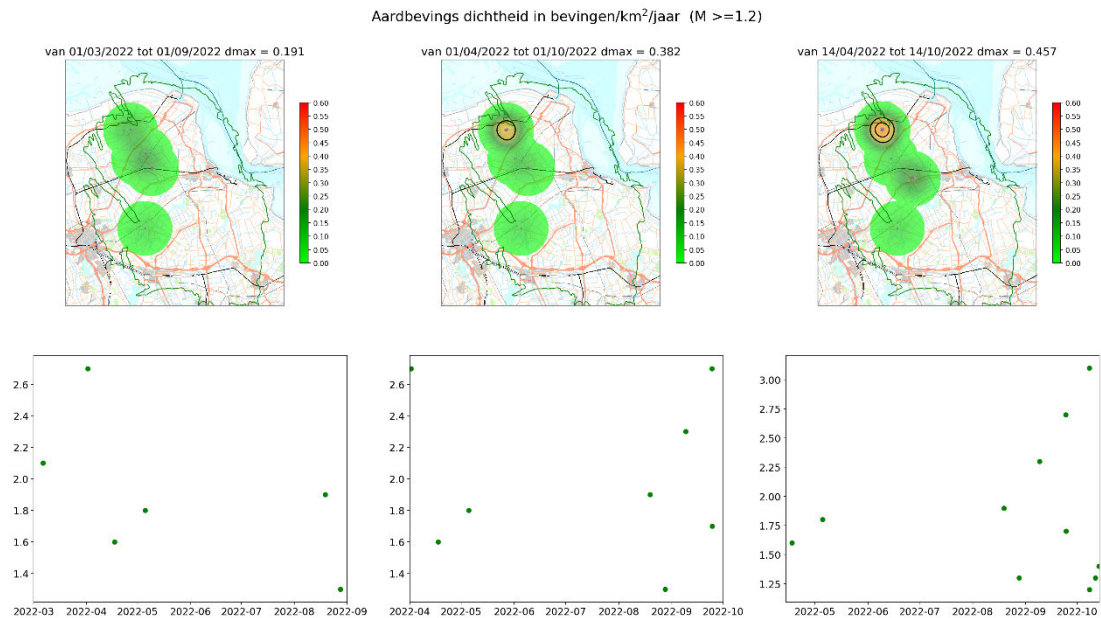
Figure 2.3 Top: Earthquake density maps for earthquakes with a magnitude larger ML \geq 1.2 during the previous six months. The earthquake density is shown as an annual density. Bottom: Graphs of earthquake magnitude versus date. Left map shows the earthquake density at 1 st September 2022. The middle map shows earthquake density at 1 st October 2022 and the right map at 14 th October 2022.
