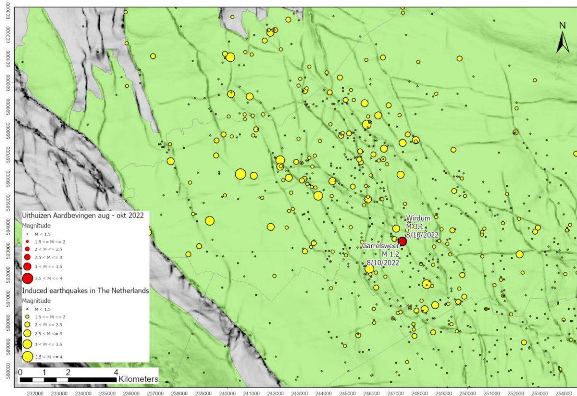
Figure 2.2 Enlargement of figure 2.1 showing the location of the earthquakes on the 8 th October 2022 near Wirdum.
