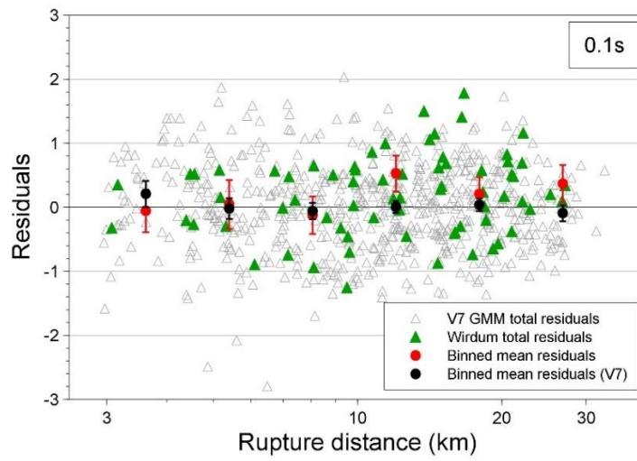
Figure 3.21 Residuals of S_a(T) with respect to the central branch of the V7 GMM at 0.1 seconds
